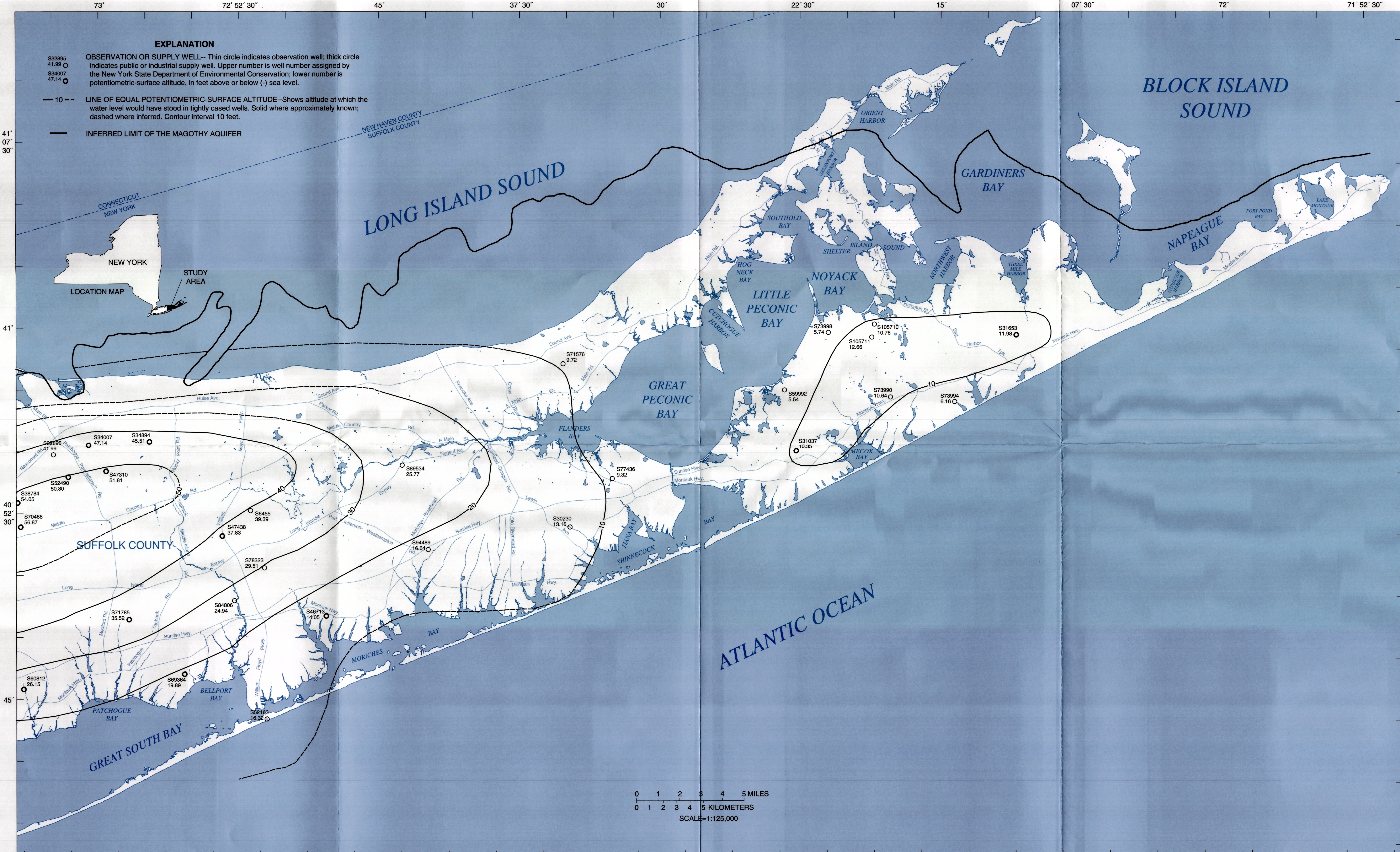
POTENTOMETRIC SURFACE OF THE MAGOTHY AQUIFER ON EASTERN LONG ISLAND, NEW YORK, IN MARCH-APRIL 1997 By Ronald Busciolano, Jack Monti, Jr., and Anthony Chu 1997
