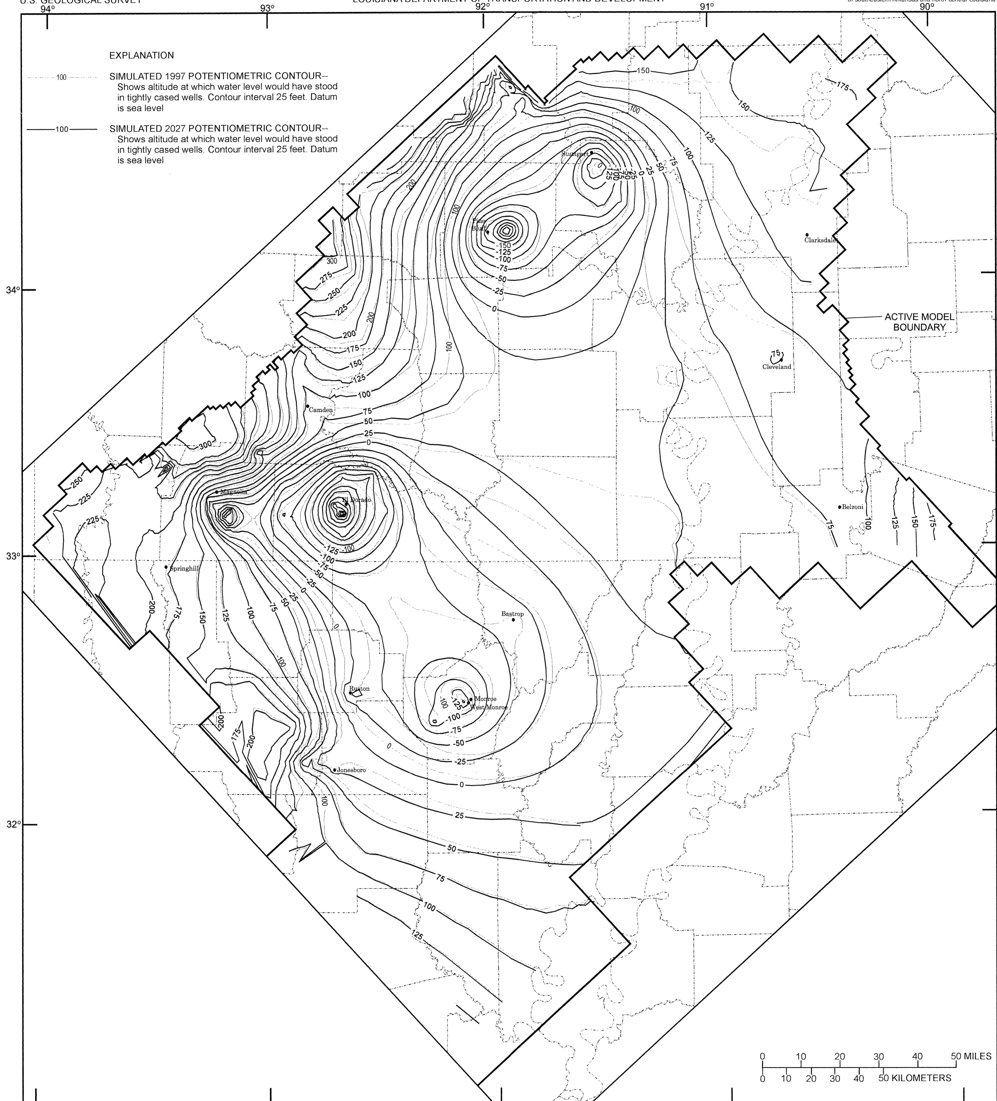
SIMULATED POTENTIOMETRIC SURFACE FOR THE SPARTA AQUIFER, 2027, SCENARIO 5 Phillip D. Hays, John Lovelace, and Thomas B. Reed 1998
