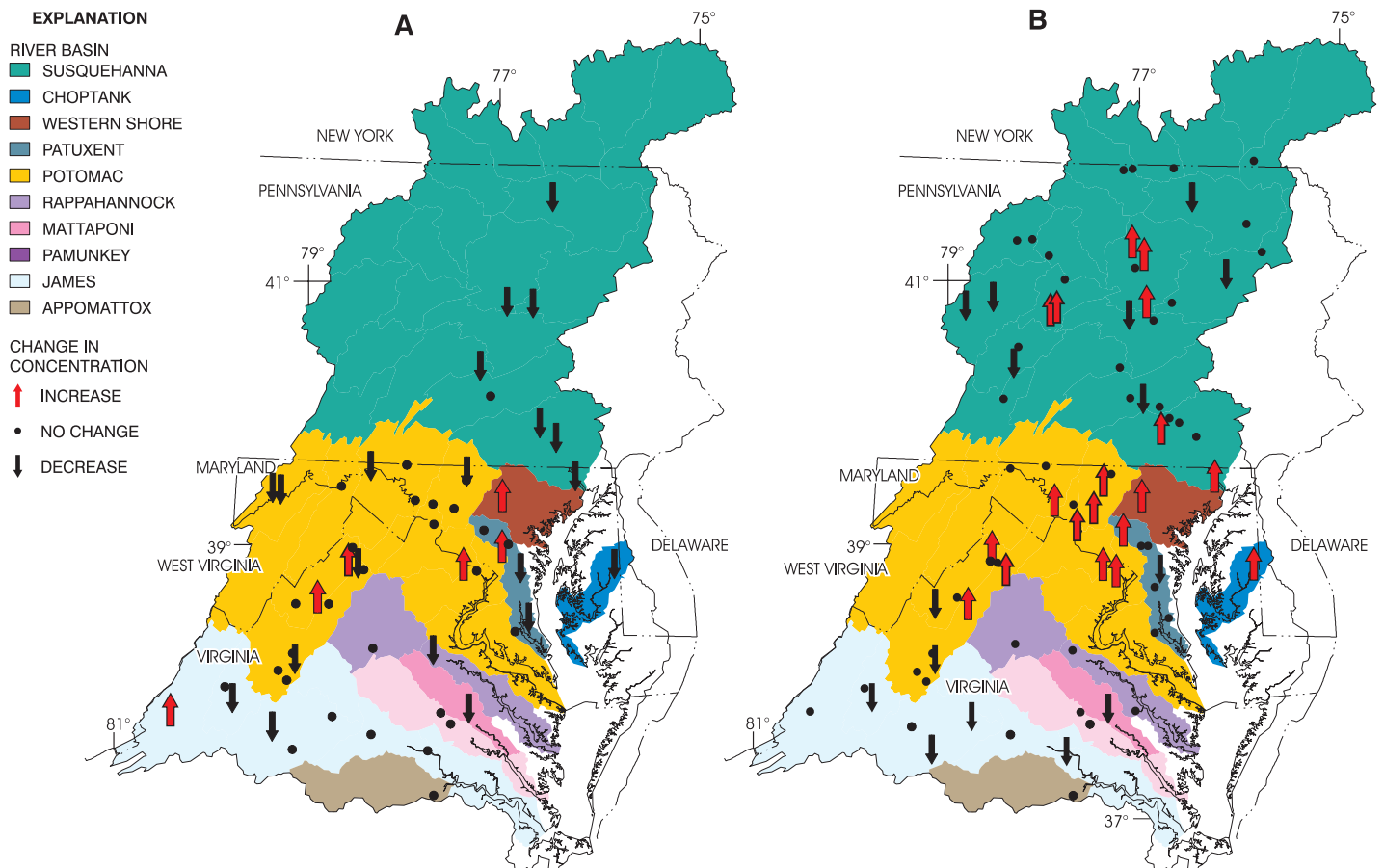
Figure 2. Trends in flow-adjusted concentrations of (A) total nitrogen, and (B) nitrate at stream sites in the Chesapeake Bay Basin.
