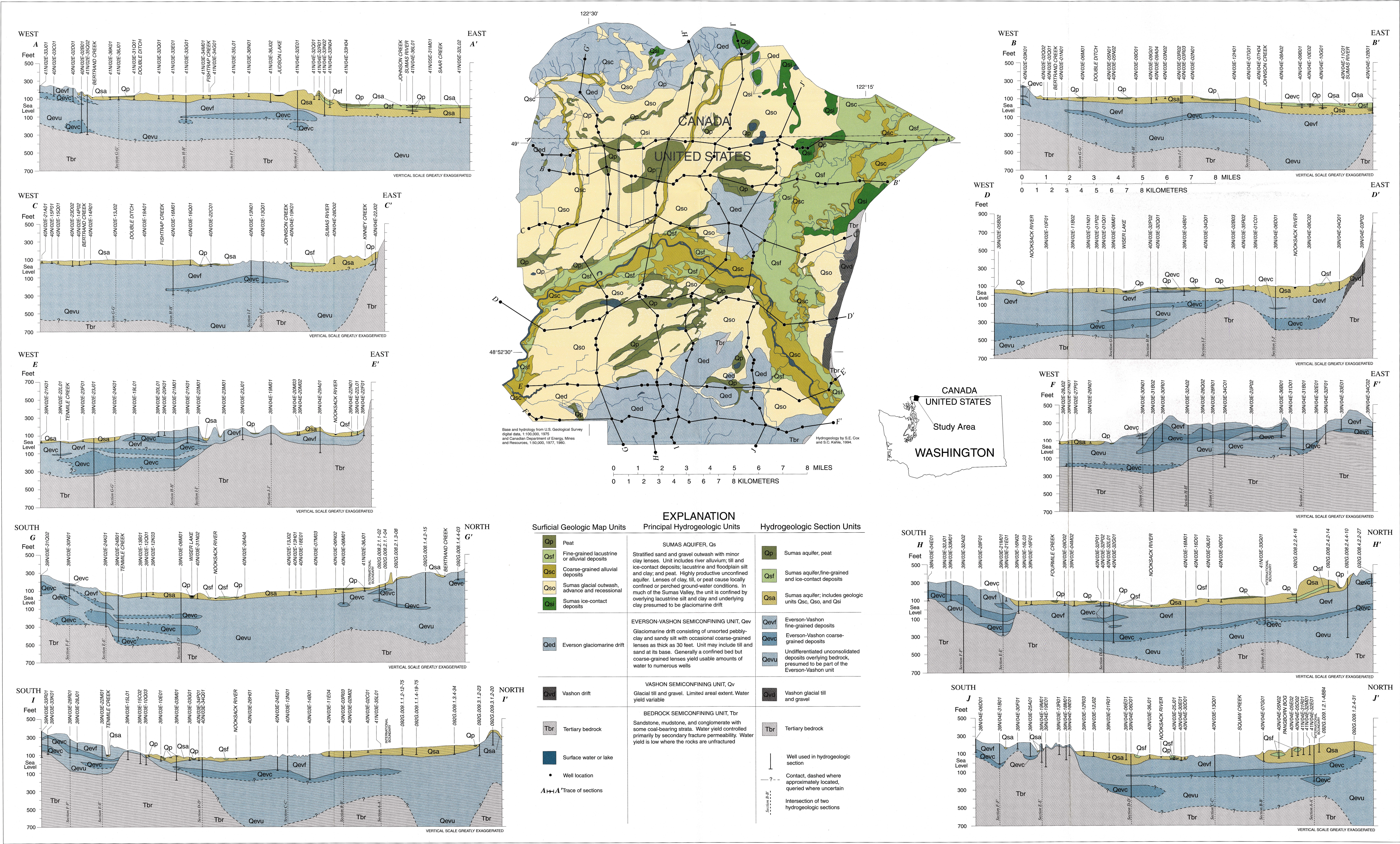
SURFICIAL GEOLOGY AND HYDROGEOLOGIC SECTIONS IN LOWLAND AQUIFERS OF WHATCOM COUNTY, WASHINGTON, AND SOUTHWESTERN BRITISH COLUMBIA
