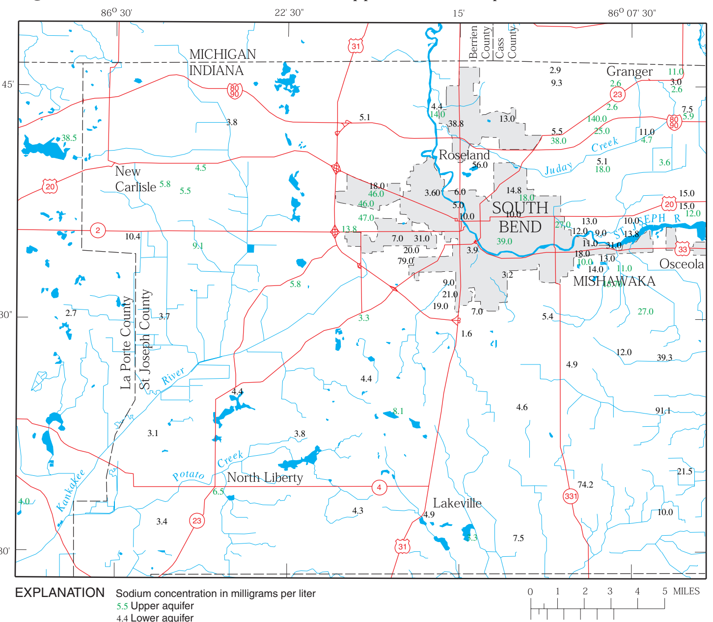
Figure 14. Concentrations of sodium in the upper and lower aquifers.
