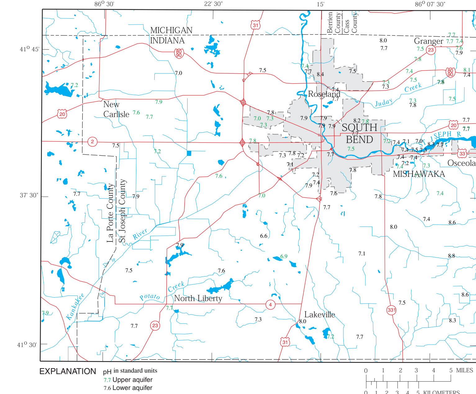
Figure 10. pH in the upper and lower aquifers.
