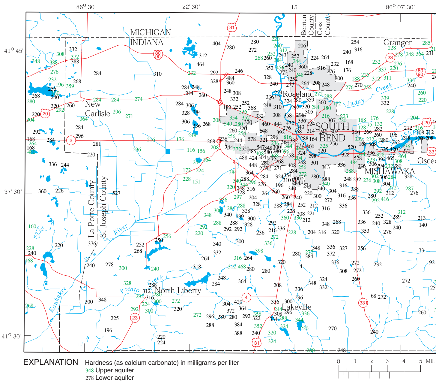
Figure 12. Hardness in the upper and lower aquifers.
