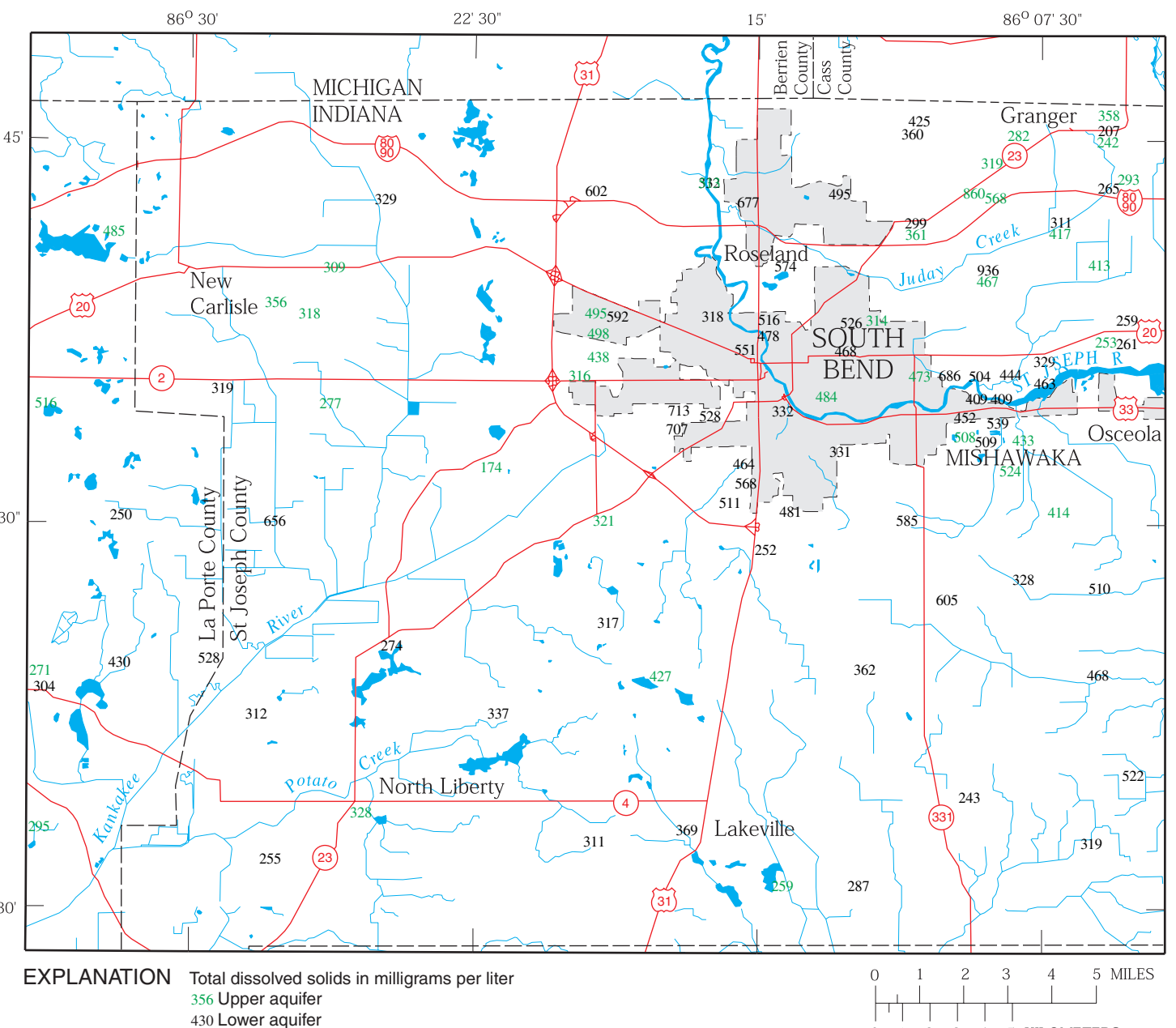
Figure 11. Total dissolved solids in the upper and lower aquifers.
