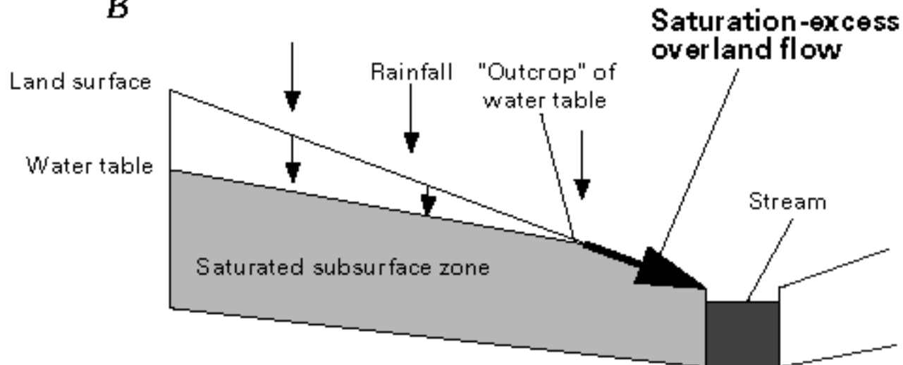
Figure 2. Schematic diagrams illustrating (A) infiltration-excess overland flow and (B) saturation-excess overland flow.
