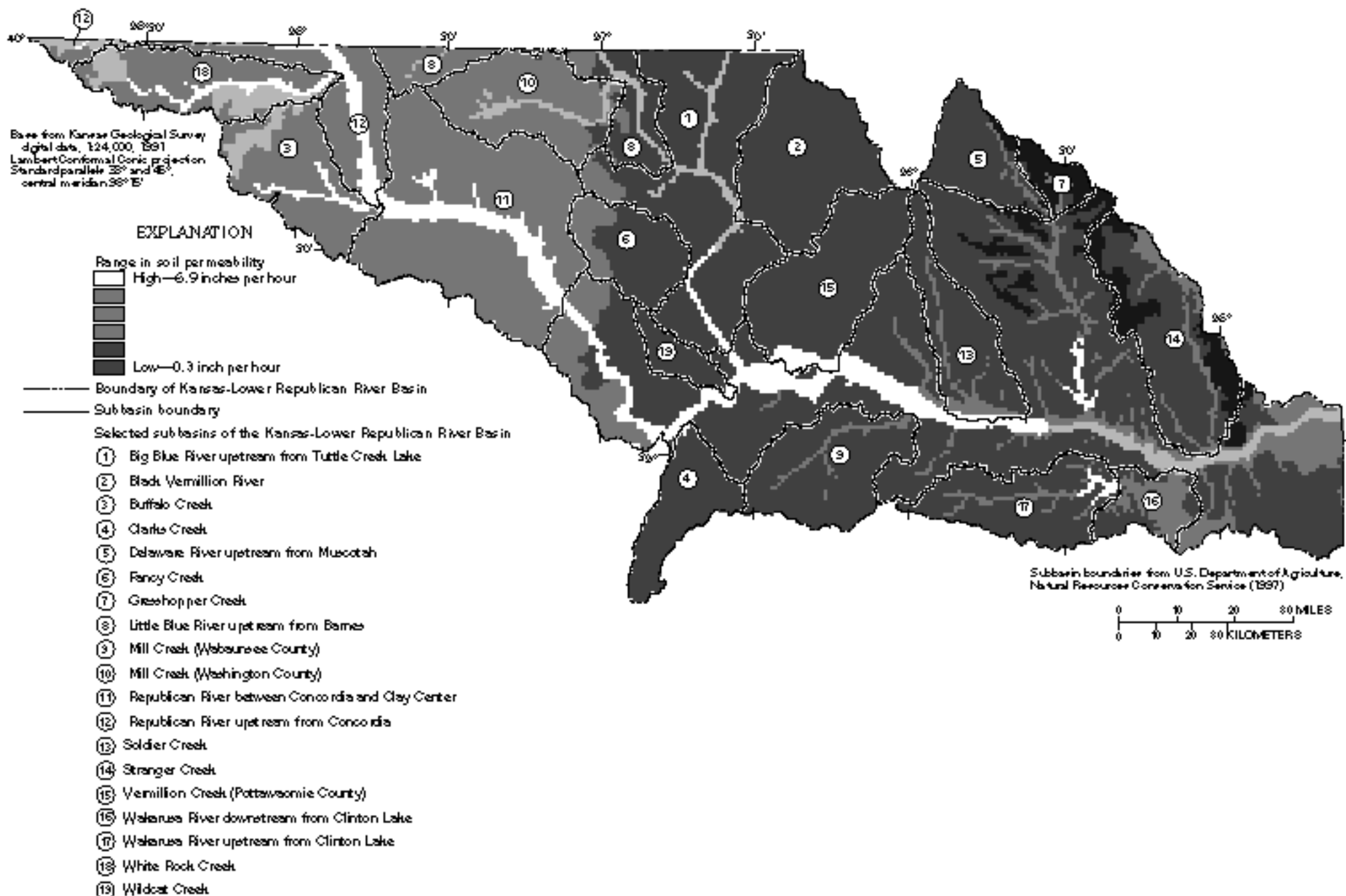
Figure 3. Soil permeability in the Kansas-Lower Republican River Basin (source of soil-permeability data: U.S. Department of Agriculture, 1993).
