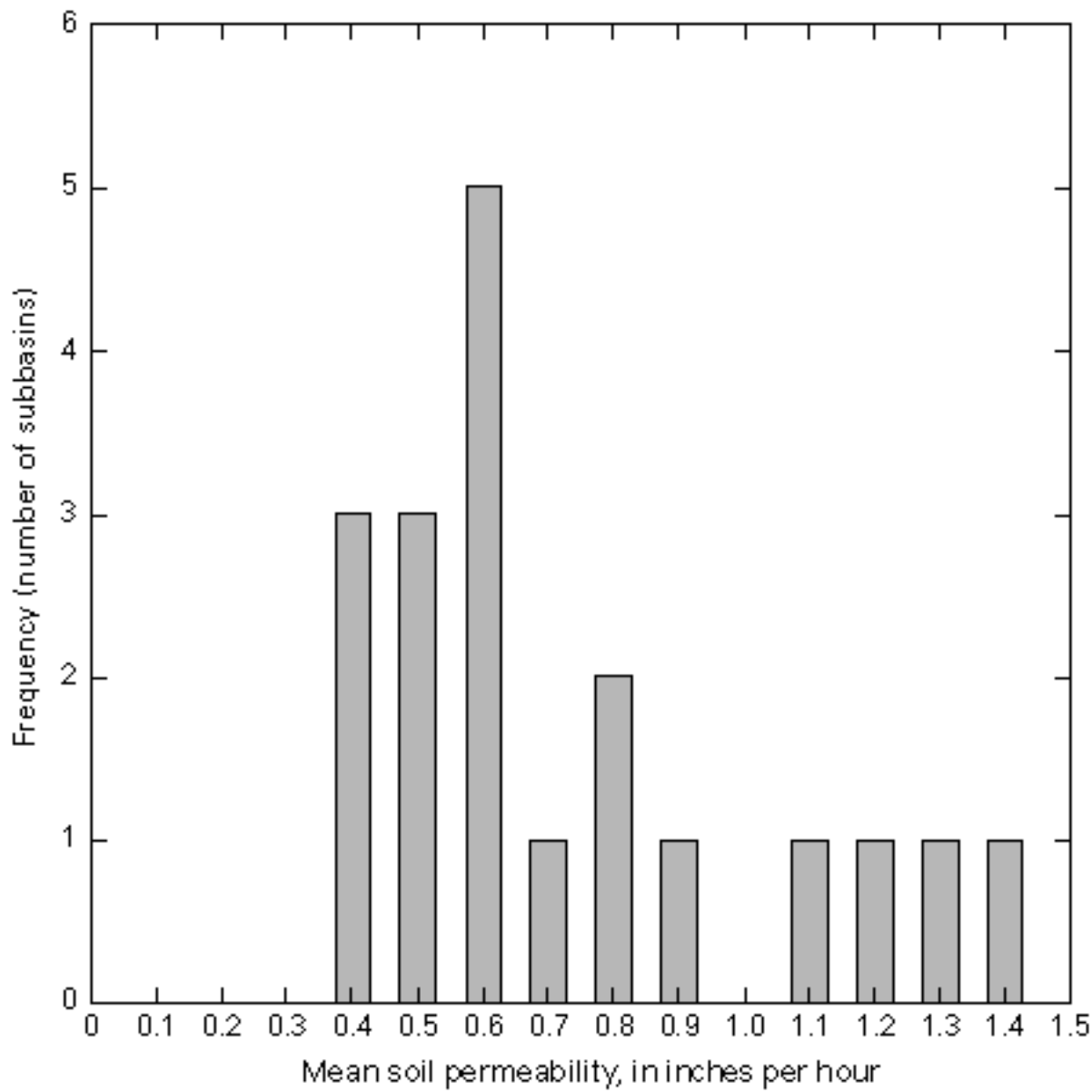
Figure 6. Frequency distribution of mean soil permeabilities for selected Kansas-Lower Republican River subbasins.
