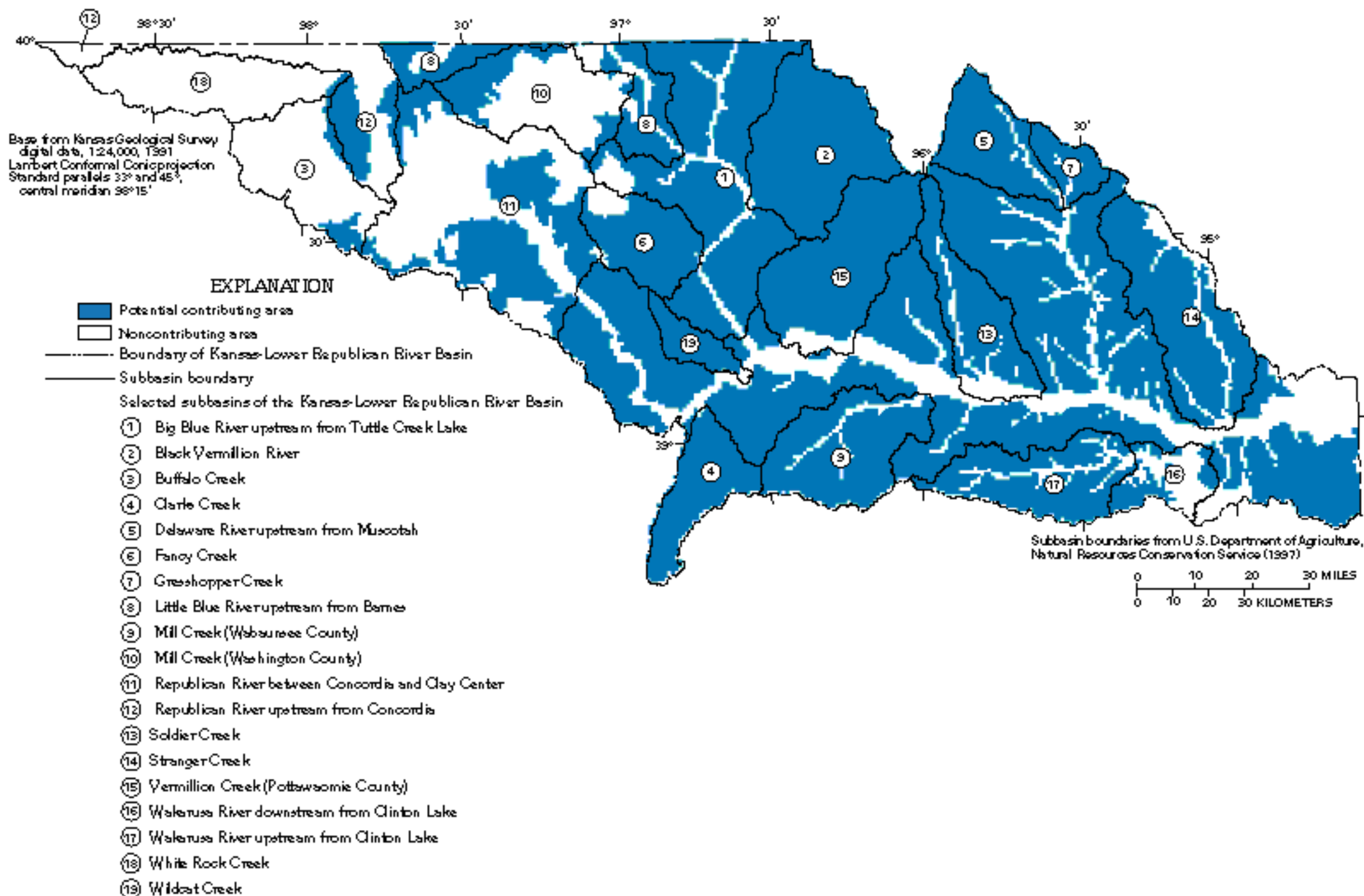
Figure 8. Potential contributing and noncontributing areas of infiltration-excess overland flow in the Kansas-Lower Republican River Basin for moderate rainfall-intensity conditions (soil permeability less than or equal to 0.80 in/hr).
