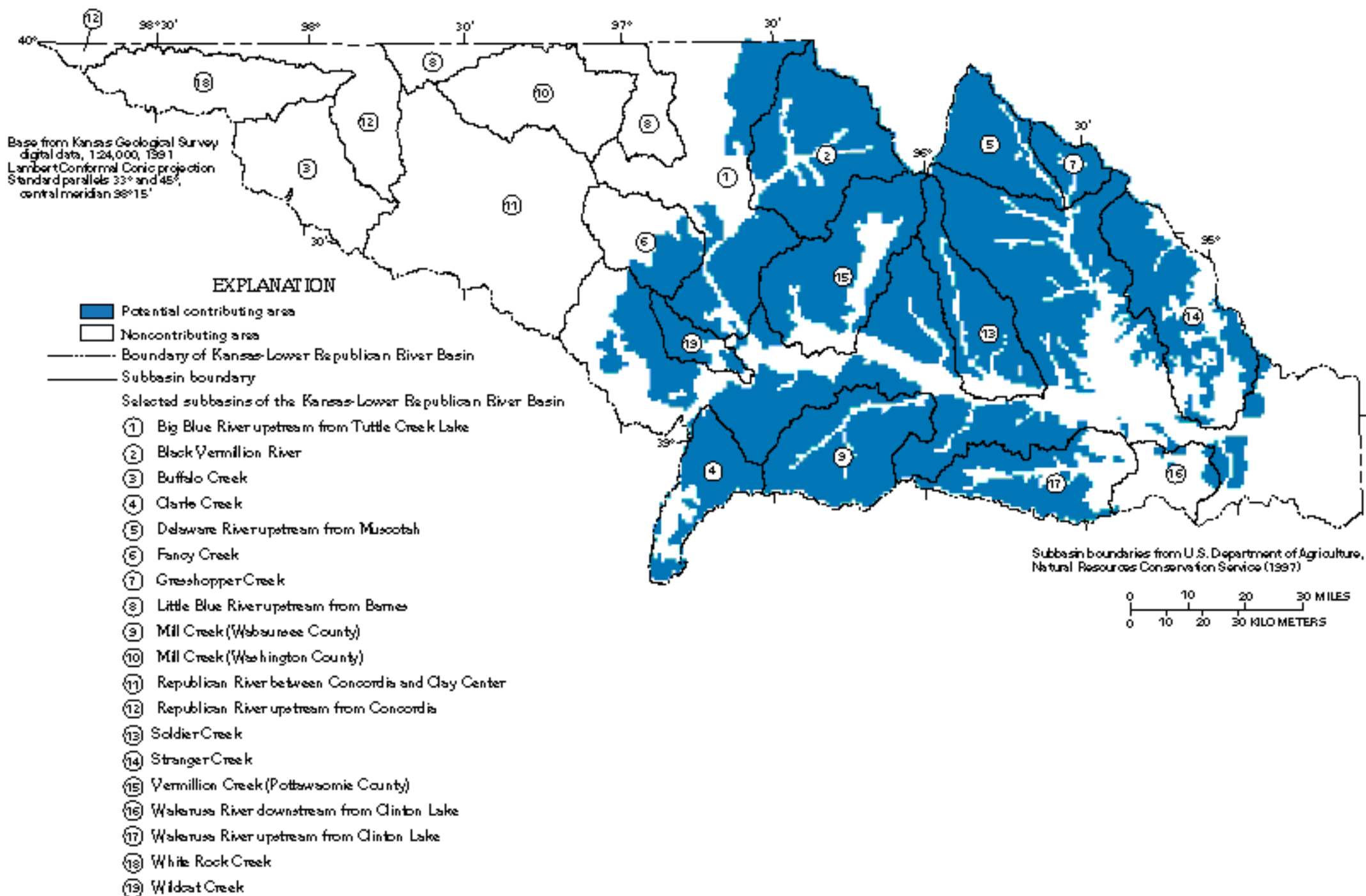
Figure 9. Potential contributing and noncontributing areas of infiltration-excess overland flow in the Kansas-Lower Republican River Basin for low rainfall-intensity conditions (soil permeability less than or equal to 0.55 in/hr).
