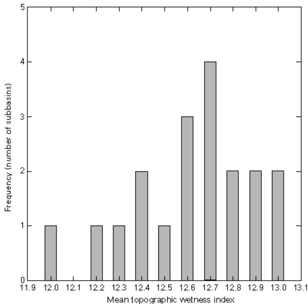
Figure 10. Frequency distribution of mean topographic wetness indices (TWI) for selected Kansas-Lower Republican River subbasins.
