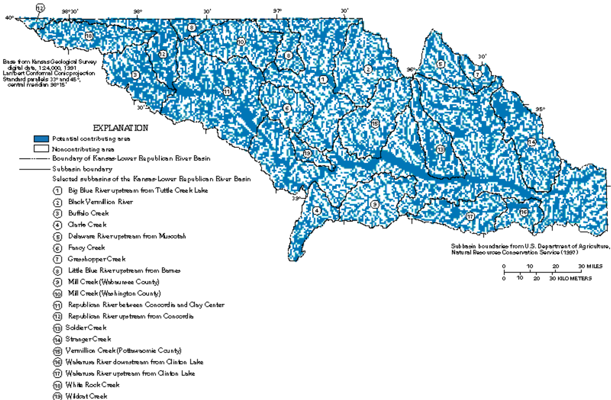
Figure 11. Potential contributing and noncontributing areas of saturation-excess overland flow in the Kansas-Lower Republican River Basin for wet antecedent soil-moisture conditions (topographic wetness index greater than or equal to 11.3).
