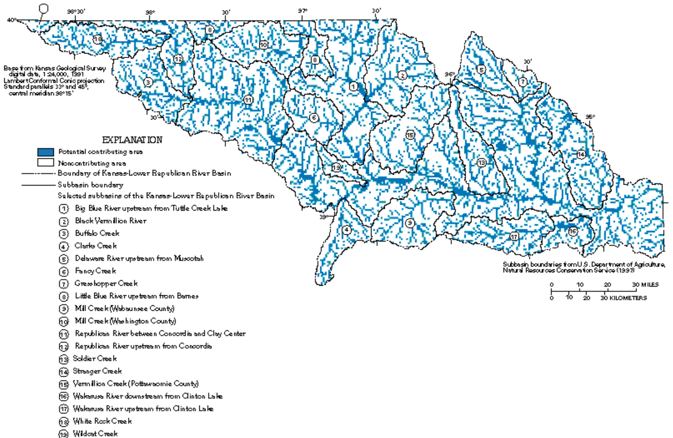
Figure 12. Potential contributing and noncontributing areas of saturation-excess overland flow in the Kansas-Lower Republican River Basin for moderate antecedent soil-moisture conditions (topographic wetness index greater than or equal to 13.9).
