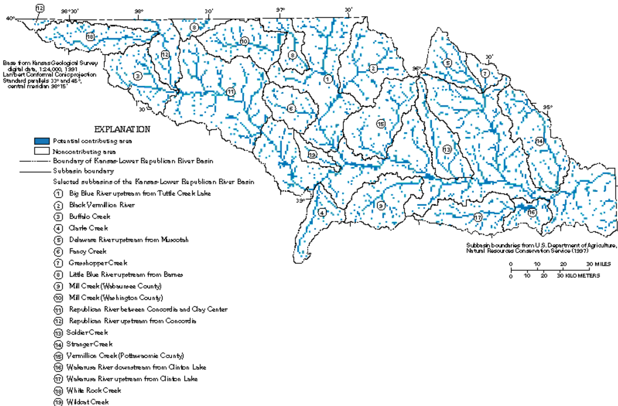
Figure 13. Potential contributing and noncontributing areas of saturation-excess overland flow in the Kansas-Lower Republican River Basin for dry antecedent soil-moisture conditions (topographic wetness index greater than or equal to 16.4).
