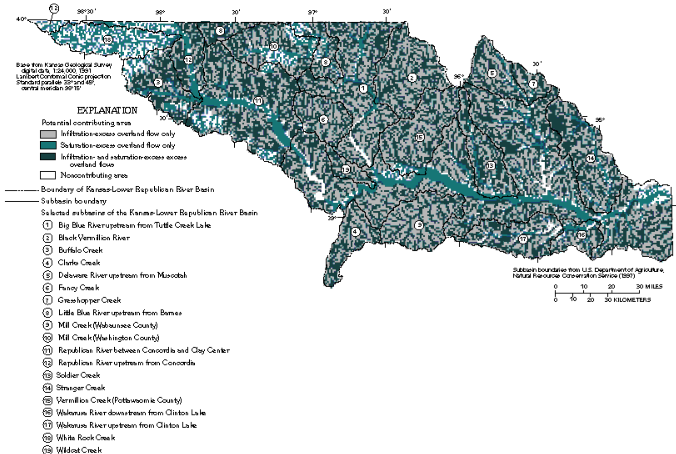
Figure 14. Potential contributing and noncontributing areas of combined infiltration- and saturation-excess overland flows in the Kansas-Lower Republican River Basin for high potential-runoff conditions (soil permeability less than or equal to 1.05 in/yr, topographic wetness index greater than or equal to 11.3).
