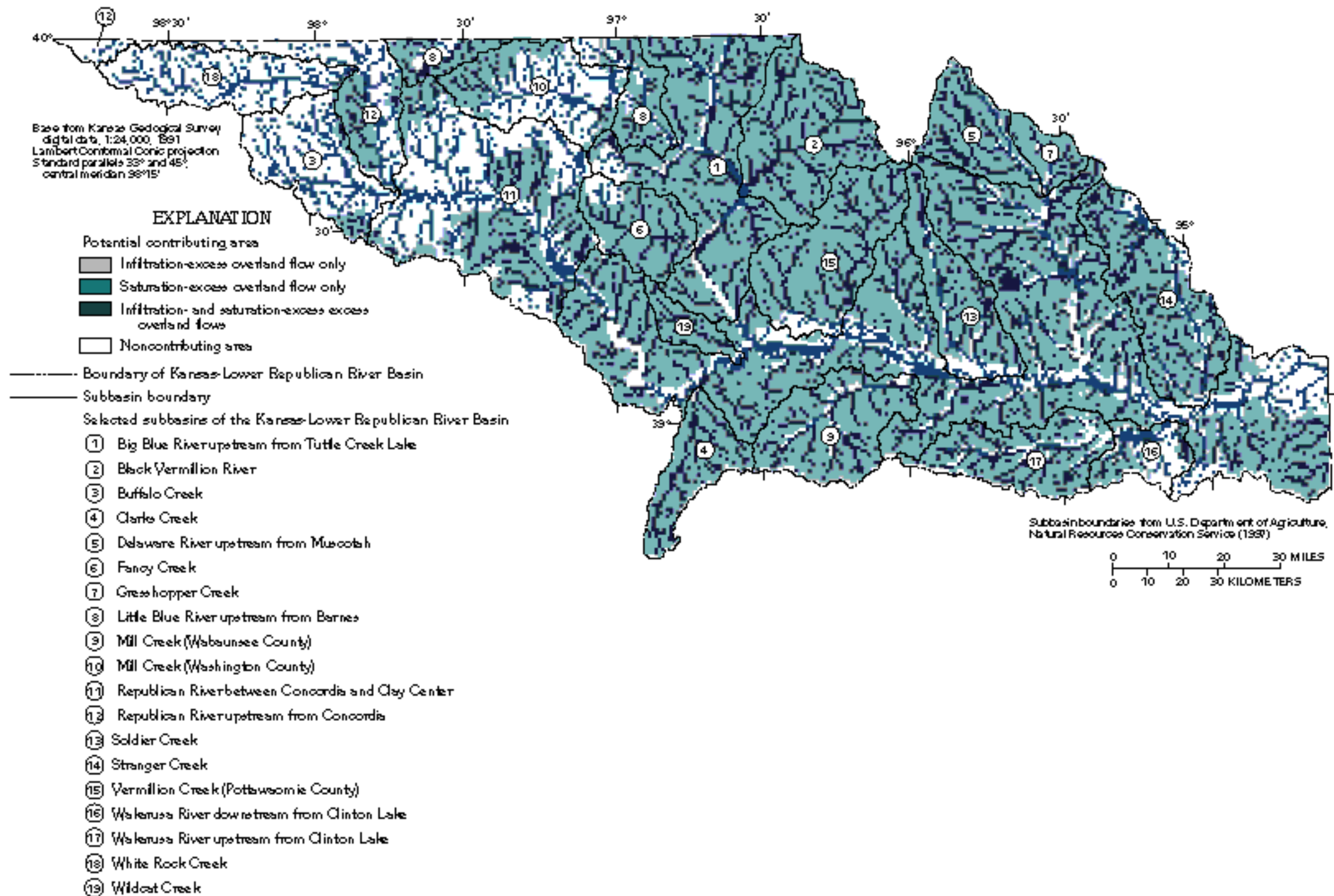
Figure 15. Potential contributing and noncontributing areas of combined infiltration- and saturation-excess overland flows in the Kansas-Lower Republican River Basin for moderate potential-runoff conditions (soil permeability less than or equal to 0.08 in/yr, topographic wetness index greater than or equal to 13.9).
