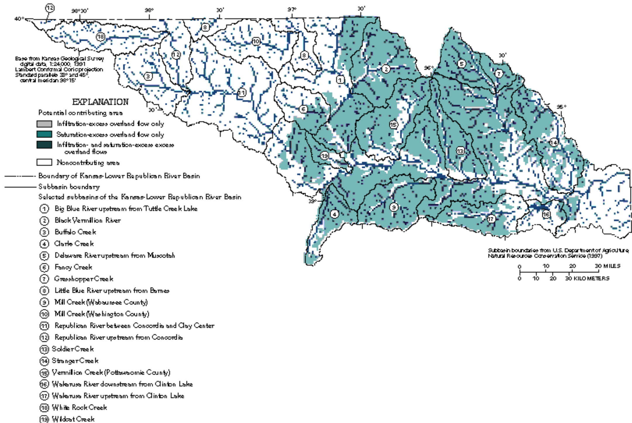
Figure 16. Potential contributing and noncontributing areas of combined infiltration- and saturation-excess overland flows in the Kansas-Lower Republican River Basin for low-potential-runoff conditions (soil permeability less than or equal to 0.55 in/yr, topographic wetness index greater than or equal to 16.4).
