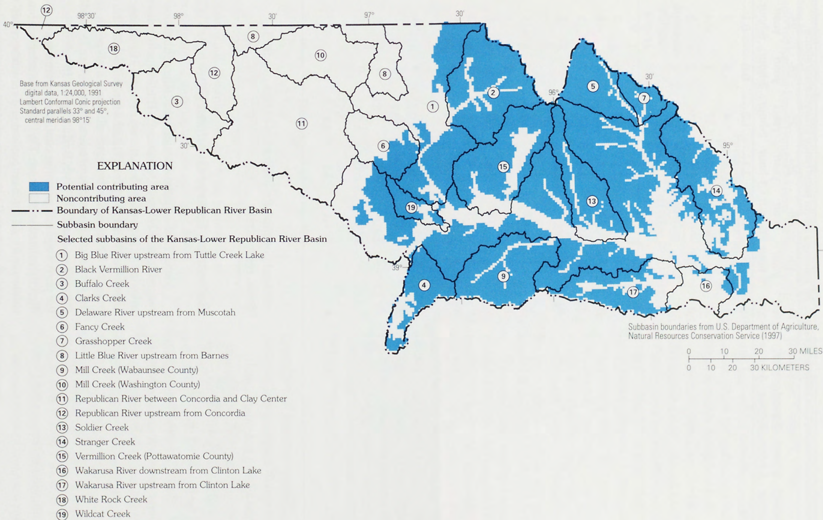
Figure 9. Potential contributing and noncontributing areas of infiltration-excess overland flow in the Kansas-Lower Republican River Basin for low rainfall-intensity conditions (soil permeability less than or equal to 0.55 in/hr).
