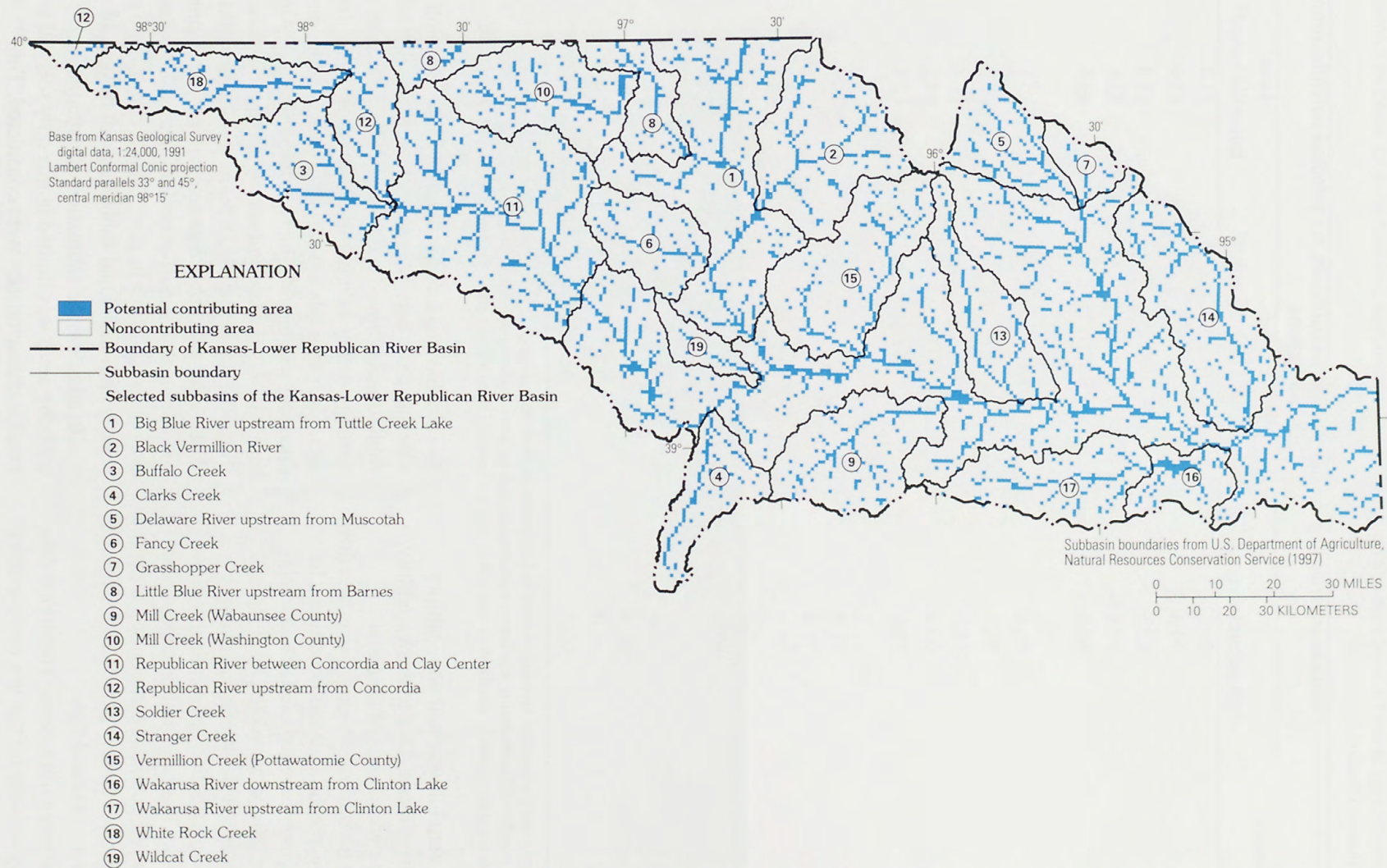
Figure 13. Potential contributing and noncontributing areas of saturation-excess overland flow in the Kansas-Lower Republican River Basin for dry antecedent soil-moisture conditions (topographic wetness index greater than or equal to 16.4).
