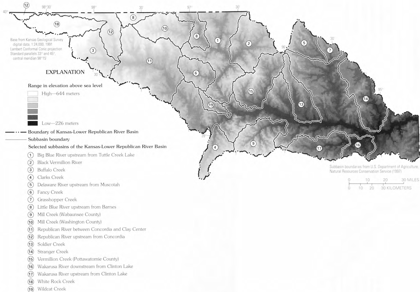
Figure 4. Digital elevation model (DEM) data for the Kansas-Lower Republican River Basin (source of DEM data: Verdin and Greenlee, 1996).
