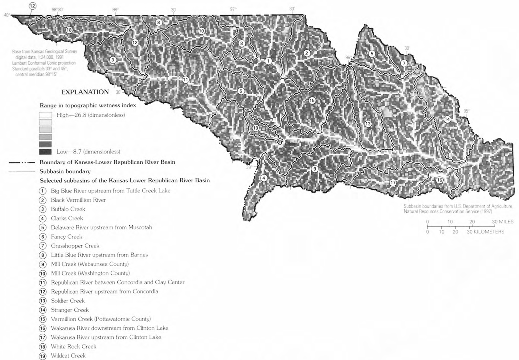
Figure 5. Topographic wetness index (TWI) data for the Kansas-Lower Republican River Basin.
