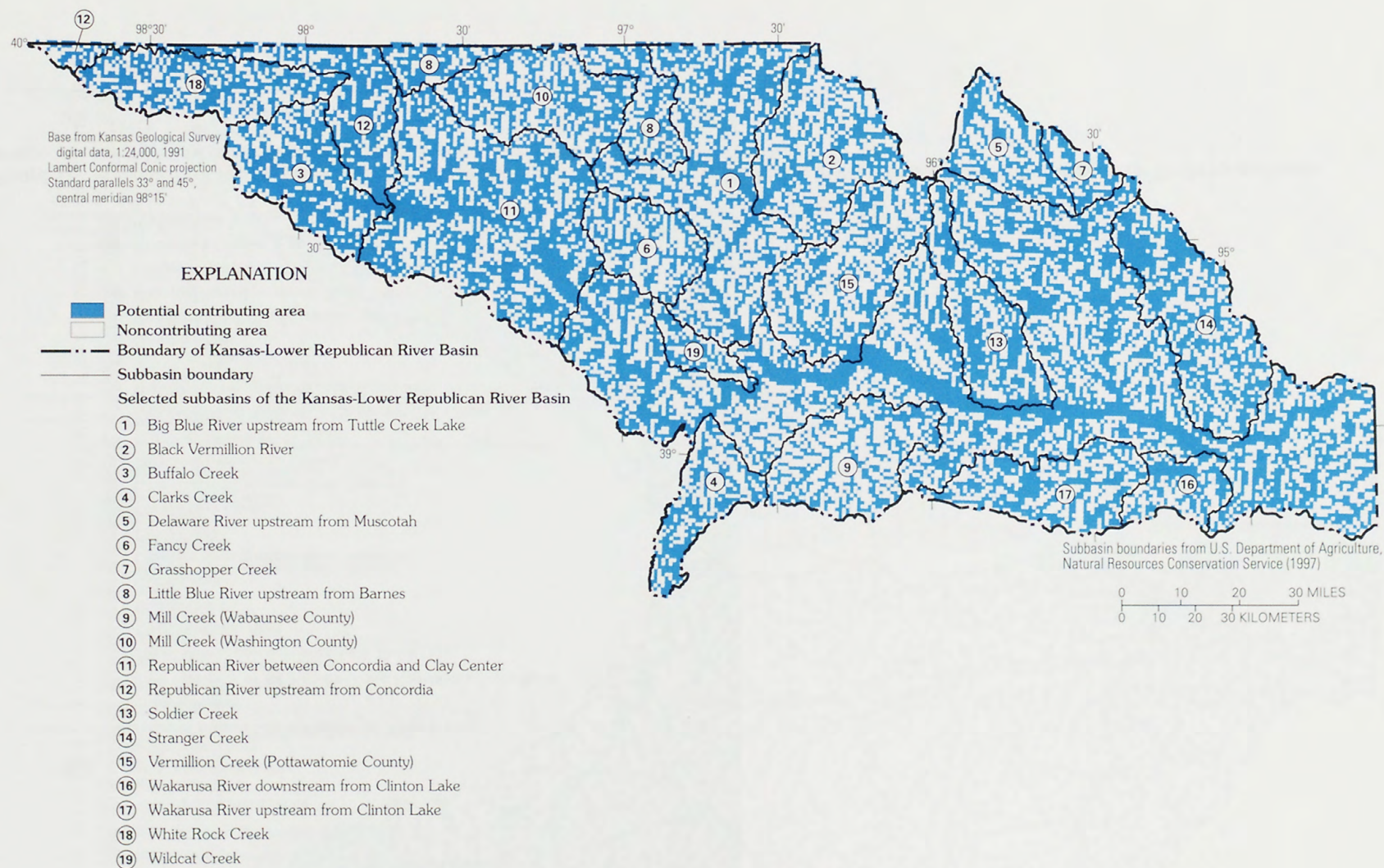
Figure 11. Potential contributing and noncontributing areas of saturation-excess overland flow in the Kansas-Lower Republican River Basin for wet antecedent soil-moisture conditions (topographic wetness index greater than or equal to 11.3).
