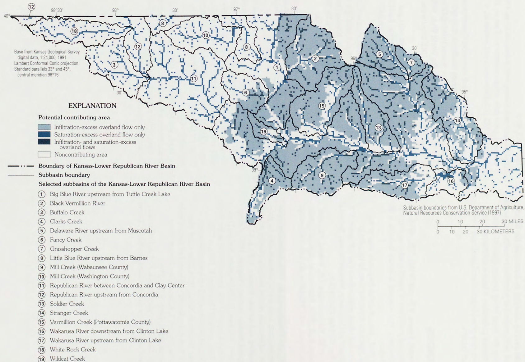
Figure 16. Potential contributing and noncontributing areas of combined infiltration- and saturation-excess overland flows in the Kansas-Lower Republican River Basin for low potential-runoff conditions (soil permeability less than or equal to 0.55 in/hr, topographic wetness index greater than or equal to 16.4).
