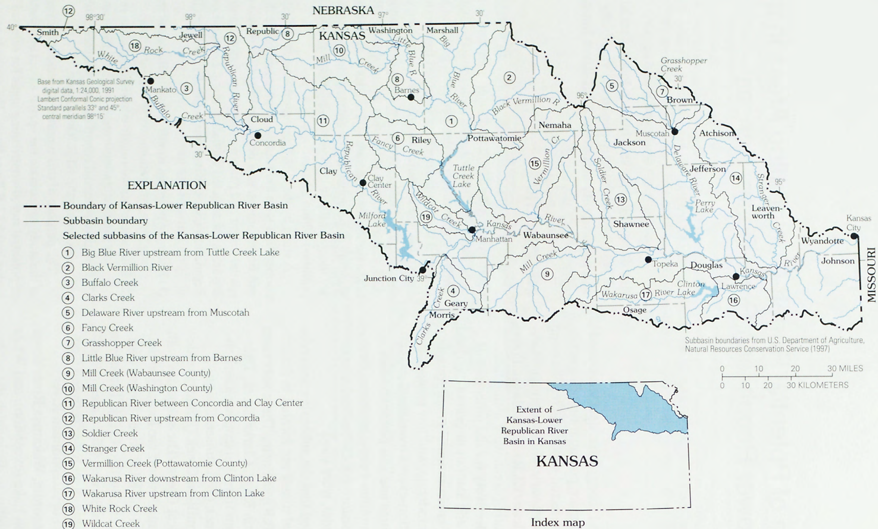
Figure 1. Location of Kansas-Lower Republican River Basin and selected subbasins in Kansas.
