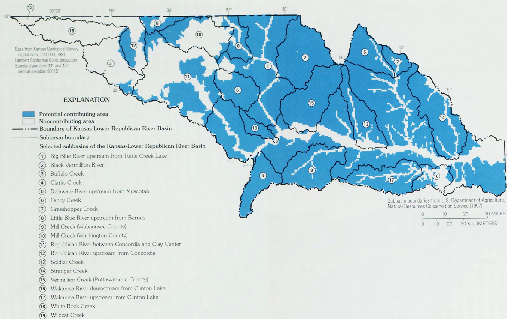
Figure 8. Potential contributing and noncontributing areas of infiltration-excess overland flow in the Kansas-Lower Republican River Basin for moderate rainfall-intensity conditions (soil permeability less than or equal to 0.80 in/hr).
