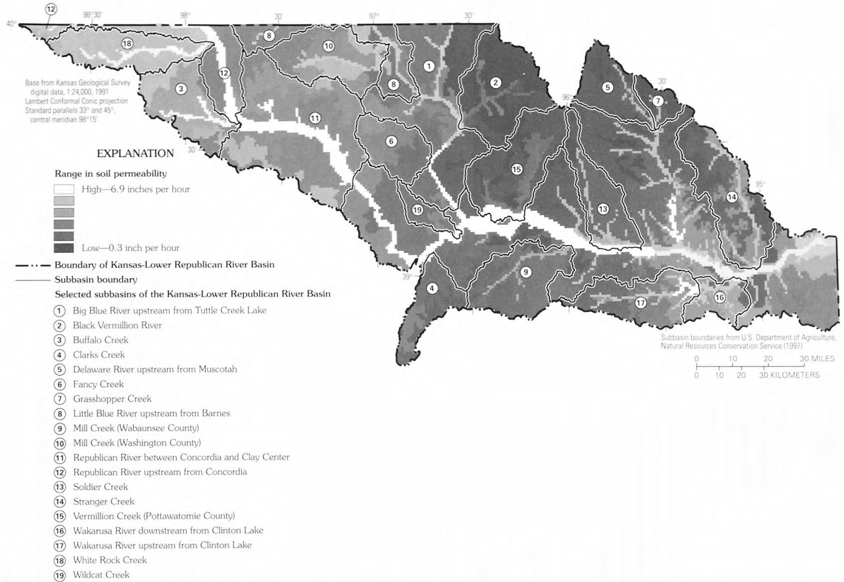
Figure 3. Soil permeability in the Kansas-Lower Republican River Basin (source of soil-permeability data: U.S. Department of Agriculture, 1993).
