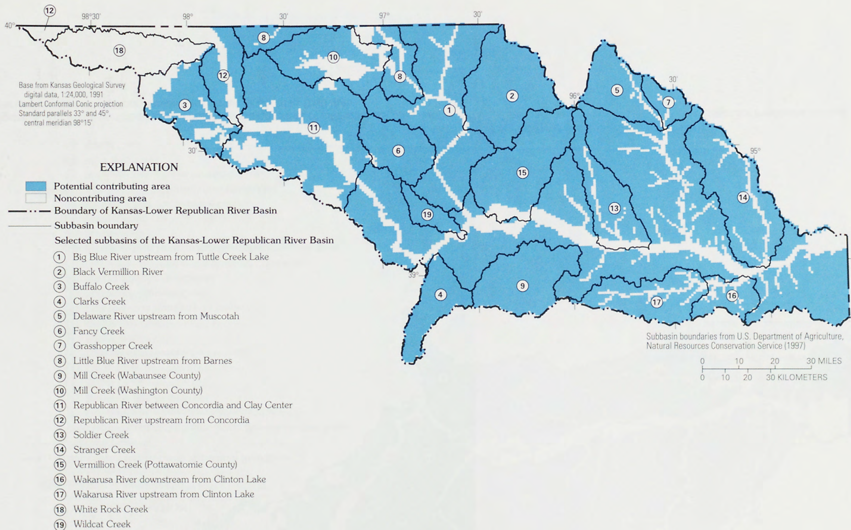
Figure 7. Potential contributing and noncontributing areas of infiltration-excess overland flow in the Kansas-Lower Republican River Basin for high rainfall-intensity conditions (soil permeability less than or equal to 1.05 in/hr).
