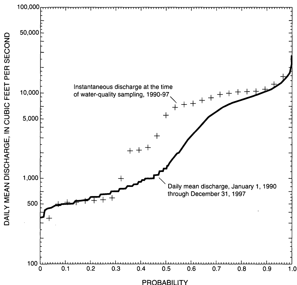
Figure 11. Cumulative probability distributions of daily mean discharge and discharge at the time of water-quality sampling of the Talkeetna River (site 41), 1990-97 (see figure 3 for location).
