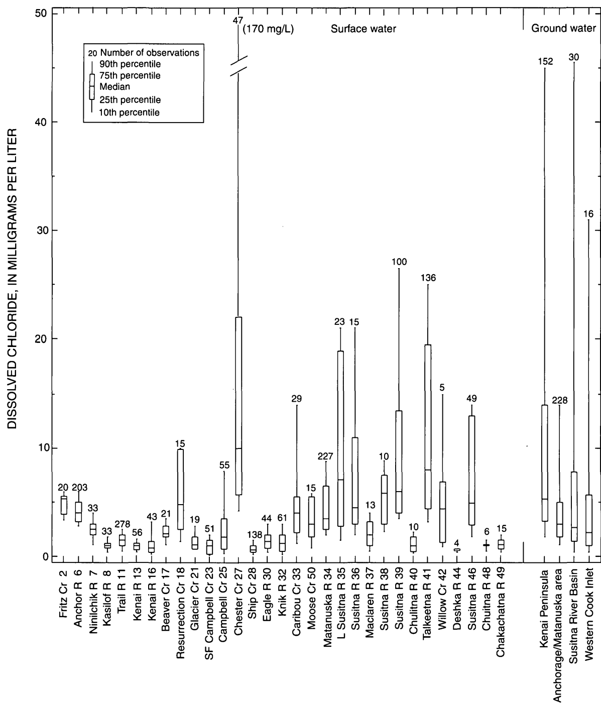
Figure 19. Dissolved-chloride concentrations in water from selected surface-water-quality monitoring sites and four ground-water regions in the Cook Inlet Basin.
