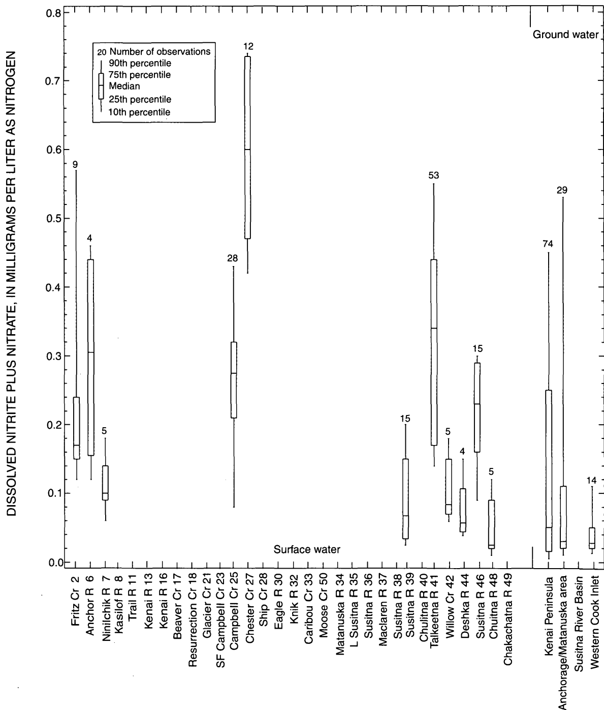
Figure 23. Dissolved nitrite plus nitrate concentrations in water from selected surface-water-quality monitoring sites and four ground-water regions in the Cook Inlet Basin.
