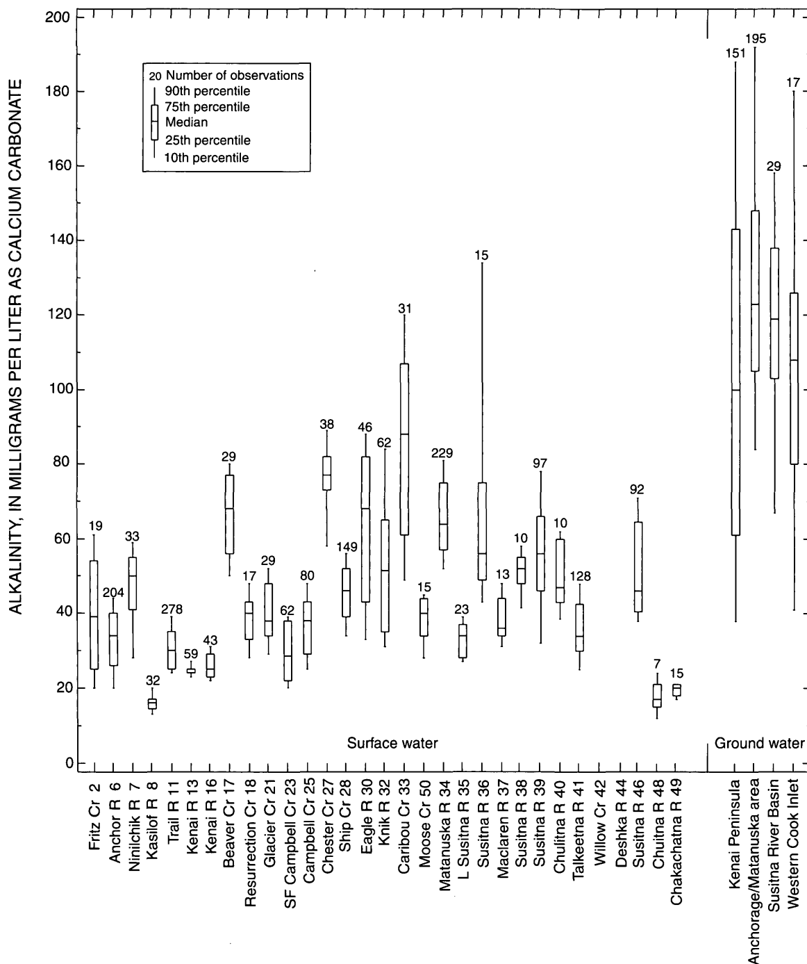
Figure 17. Alkalinity of water from selected surface-water-quality monitoring sites and four ground-water regions in the Cook Inlet Basin.
