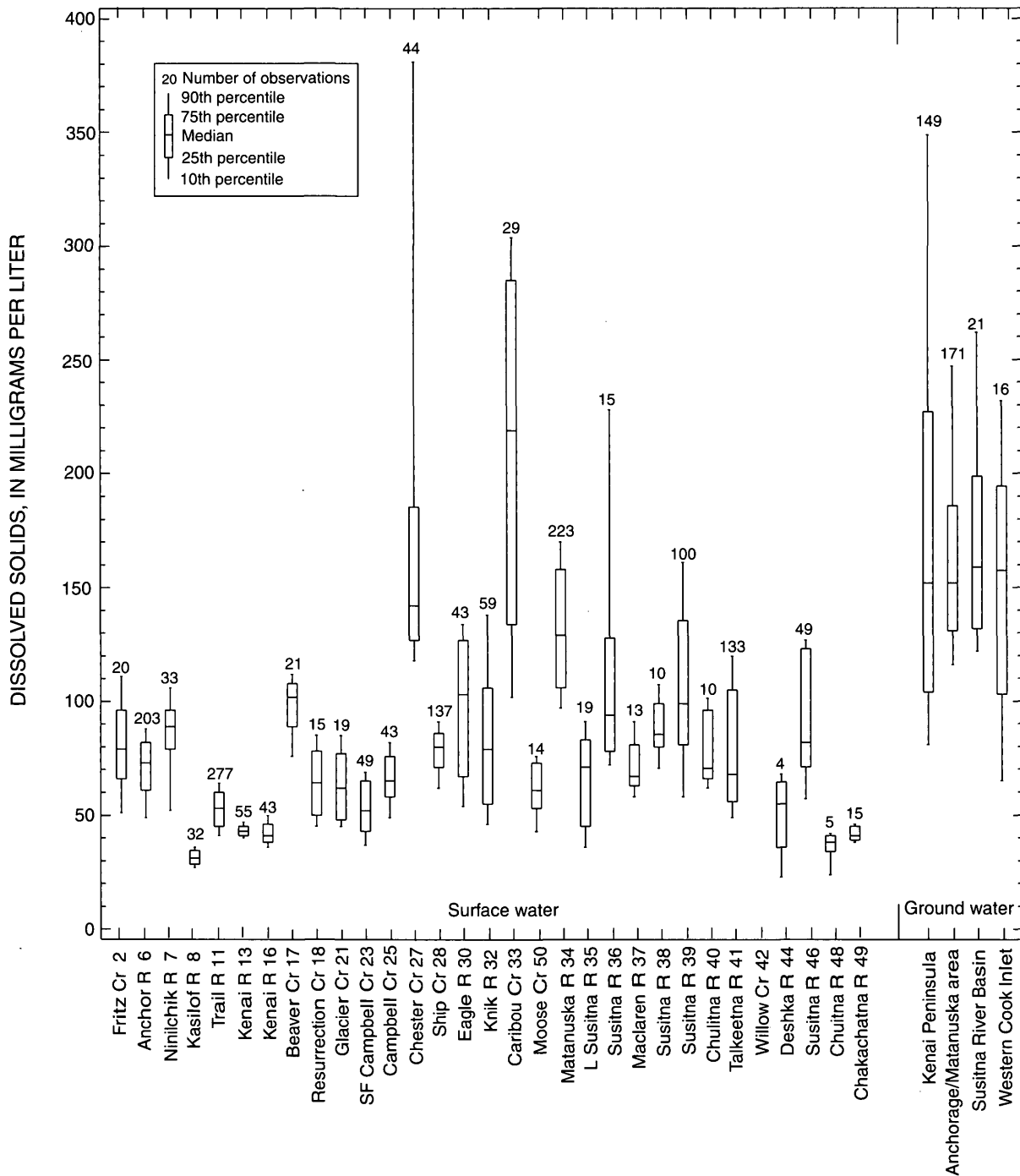
Figure 22. Dissolved-solids concentrations in water from selected surface-water-quality monitoring sites and four ground-water regions in the Cook Inlet Basin.
