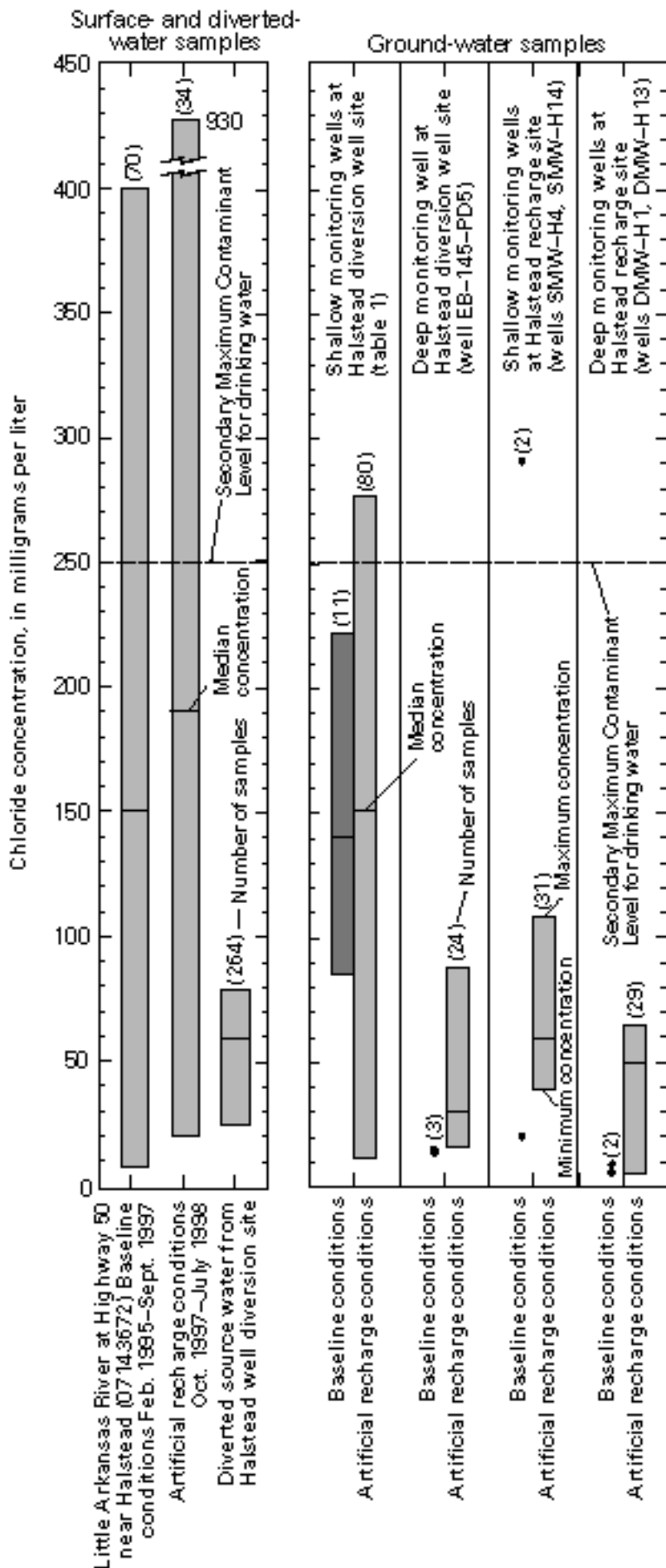
Figure 15. Ranges in chloride concentrations in surface- diverted-, and ground-water samples collected during baseline and recharge conditions. Secondary Maximum Contaminant Level from U.S. Environmental Protection Agency (1999).
