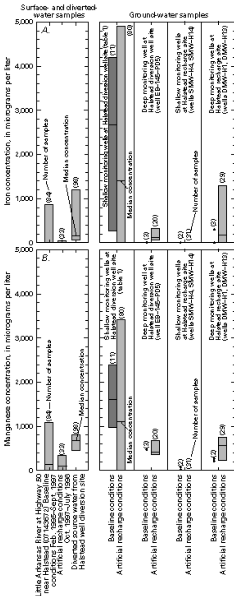
Figure 17. Ranges in (A) iron and (B) manganese concentrations in surface-, diverted-, and ground-water samples collected during baseline and recharge conditions. Secondary Maximum Contaminant Level from U.S. Environmental Protection Agency (1999).
