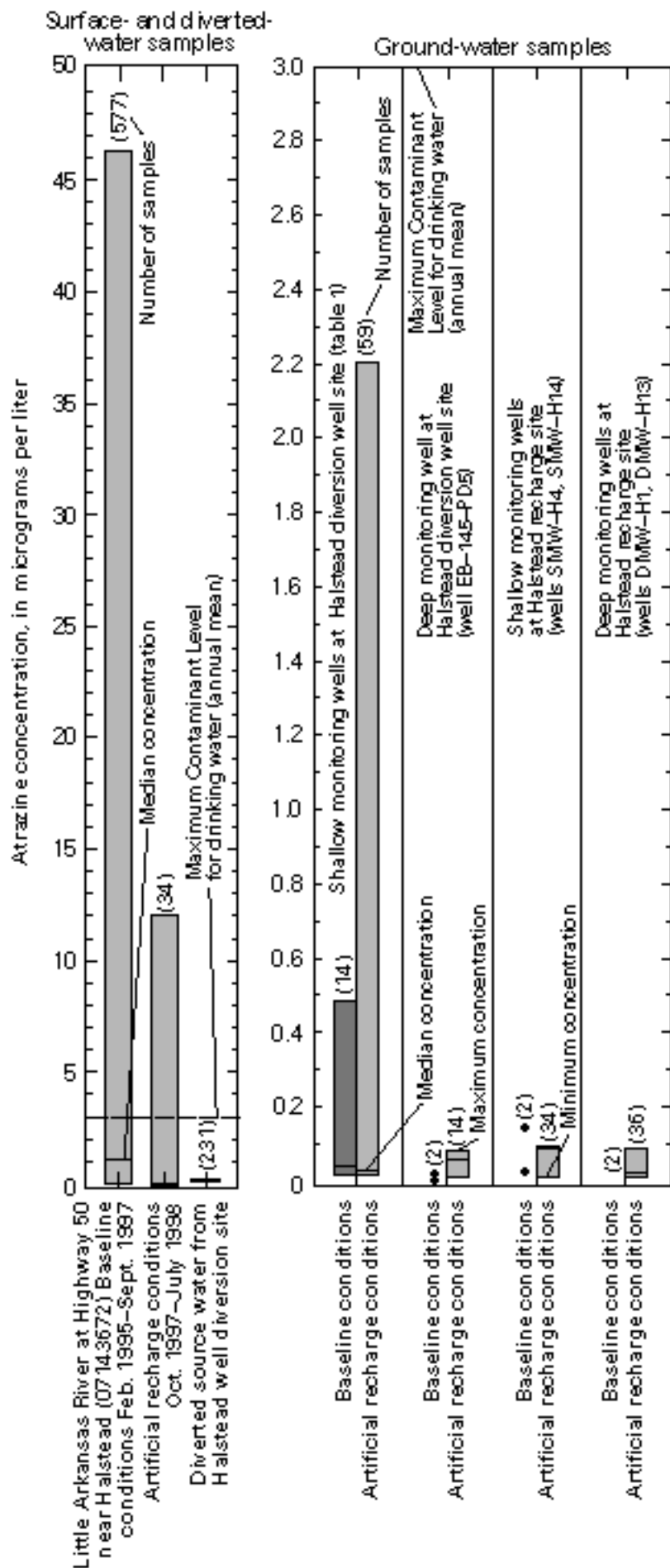
Figure 18. Ranges in atrazine concentrations in surface-diverted-, and ground-water samples collected during baseline and recharge conditions. Maximum Contaminant Level from U.S. Environmental Protection Agency (1999).
