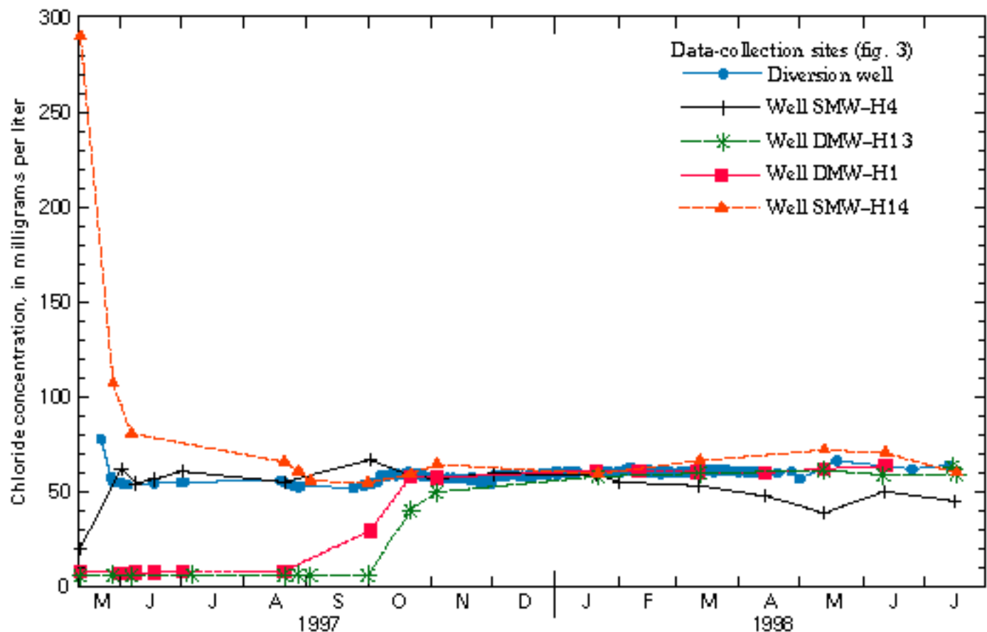
Figure 19b. Comparison of chloride concentrations (A) in surface water and ground water from Halstead diversion well site, March 1995-July 1998, and (B) in diversion well water and ground water from Halstead recharge site, May 1997-July 1998. Secondary Maximum Contaminant Level from U.S. Environmental Protection Agency (1999)-Continued.
