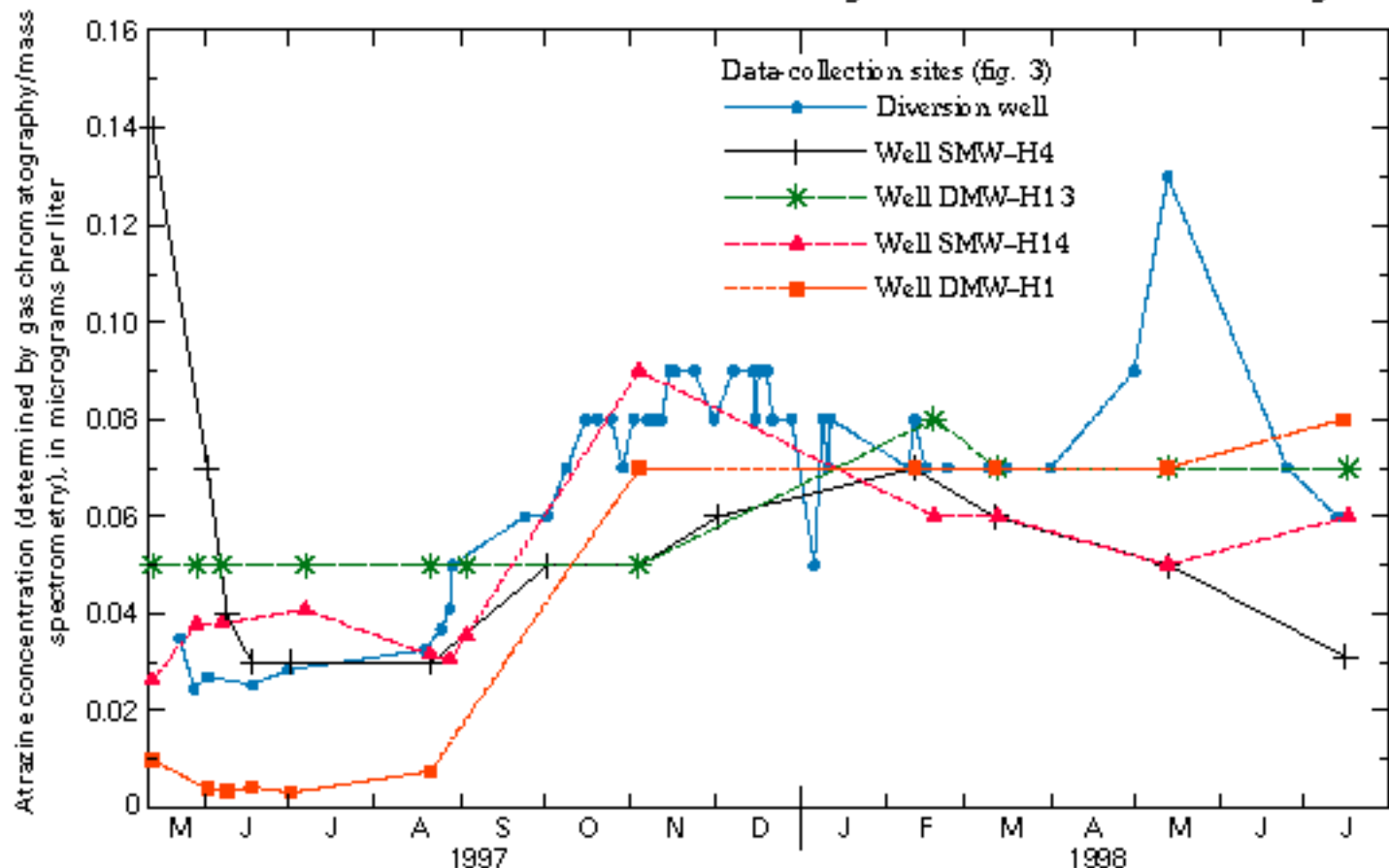
Figure 20b. Comparison of atrazine concentrations (A) in surface water and ground water from Halstead diversion well site, March 1995-July 1998, and (B) in diversion well water and ground water from Halstead recharge site, May 1997-July 1998. Maximum Contaminant Level from U.S. Environmental Protection Agency (1999)-Continued.
