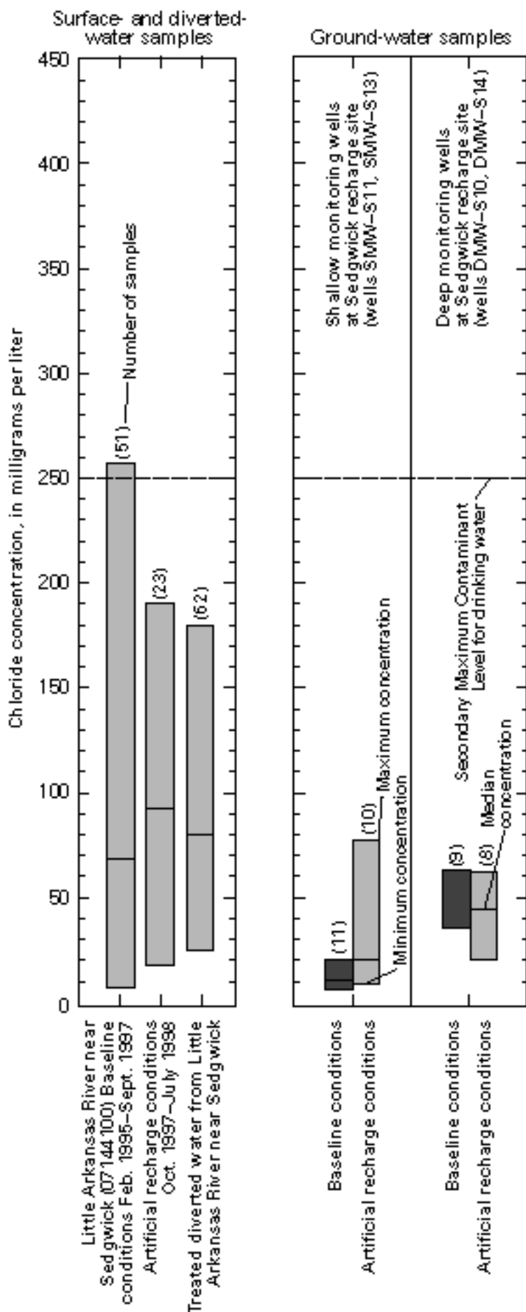
Figure 23. Ranges in chloride concentrations in surface-diverted, and ground-water samples collected during baseline and recharge conditions. Secondary Maximum Contaminant Level from U.S. Environmental Protection Agency (1999).
