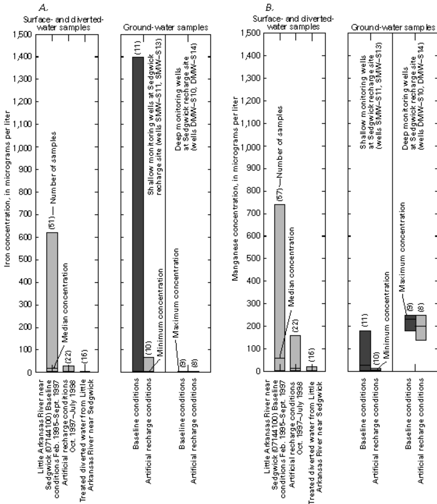
Figure 26. Ranges in (A) iron and (B) manganese concentrations in surface-, diverted, and ground-water samples collected during baseline and recharge conditions. Secondary Maximum Contaminant Level from U.S. Environmental Protection Agency (1999).
