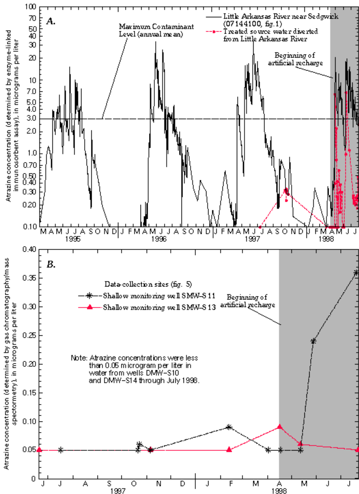
Figure 28. Comparison of atrazine concentrations in (A) surface and treated source water from Little Arkansas River, March 1995-July 1998, and in (B) water from monitoring wells at Sedgwick recharge site, June 1997-July 1998. Maximum Contaminant Level from U.S. Environmental Protection Agency (1999).
