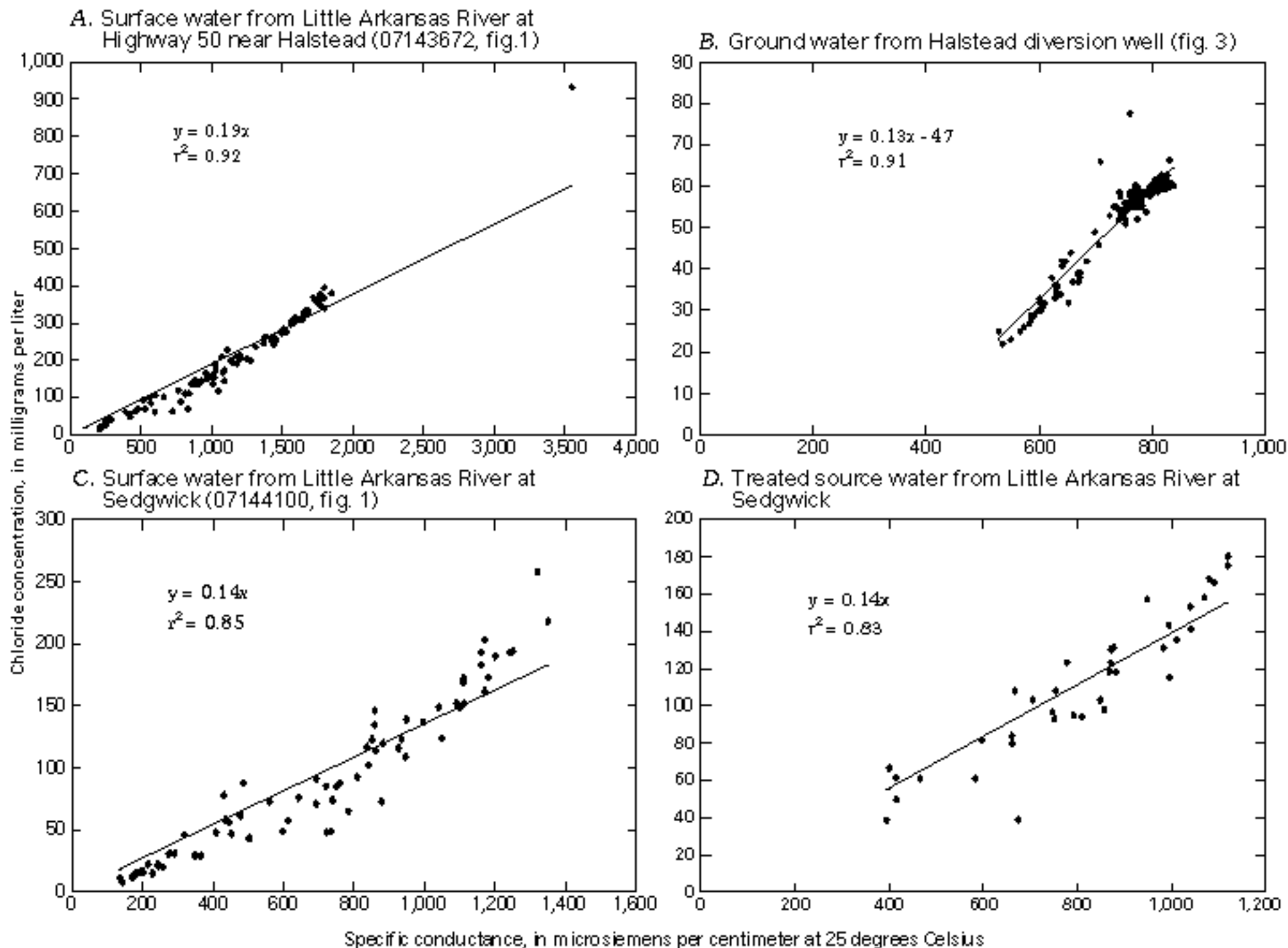
Figure 30. Relations between specific conductance and chloride concentrations in (A) surface water from Little Arkansas River at Highway 50 near Halstead, (B) ground water from Halstead diversion well, and (C) surface water and (D) treated source water from Little Arkansas River at Sedgwick, March 1995-July 1998.
