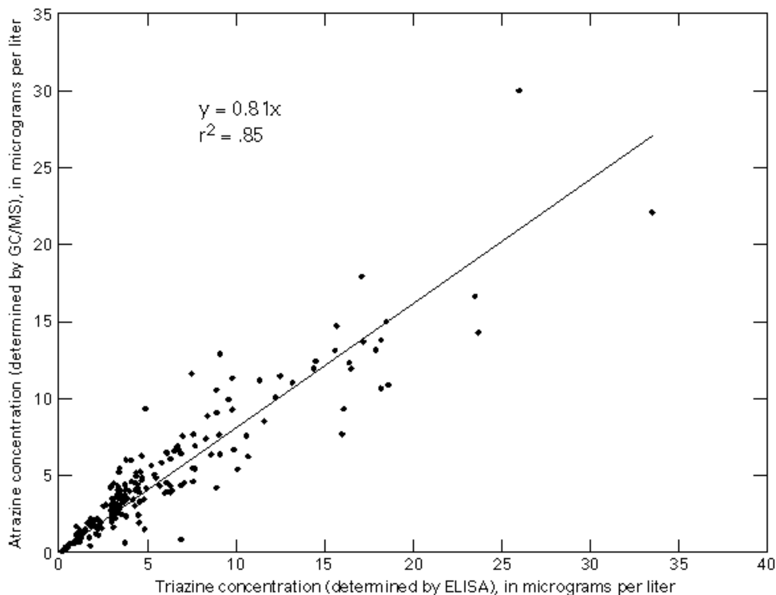
Figure 31. Relations between triazine herbicide concentrations determined by enzyme-linked immunosorbent assay (ELISA) and atrazine concentrations determined by gas chromatography/mass spectrometry (GC/MS) for samples collected from Halstead and Sedgwick surface-water monitoring sites, March 1995-July 1998.
