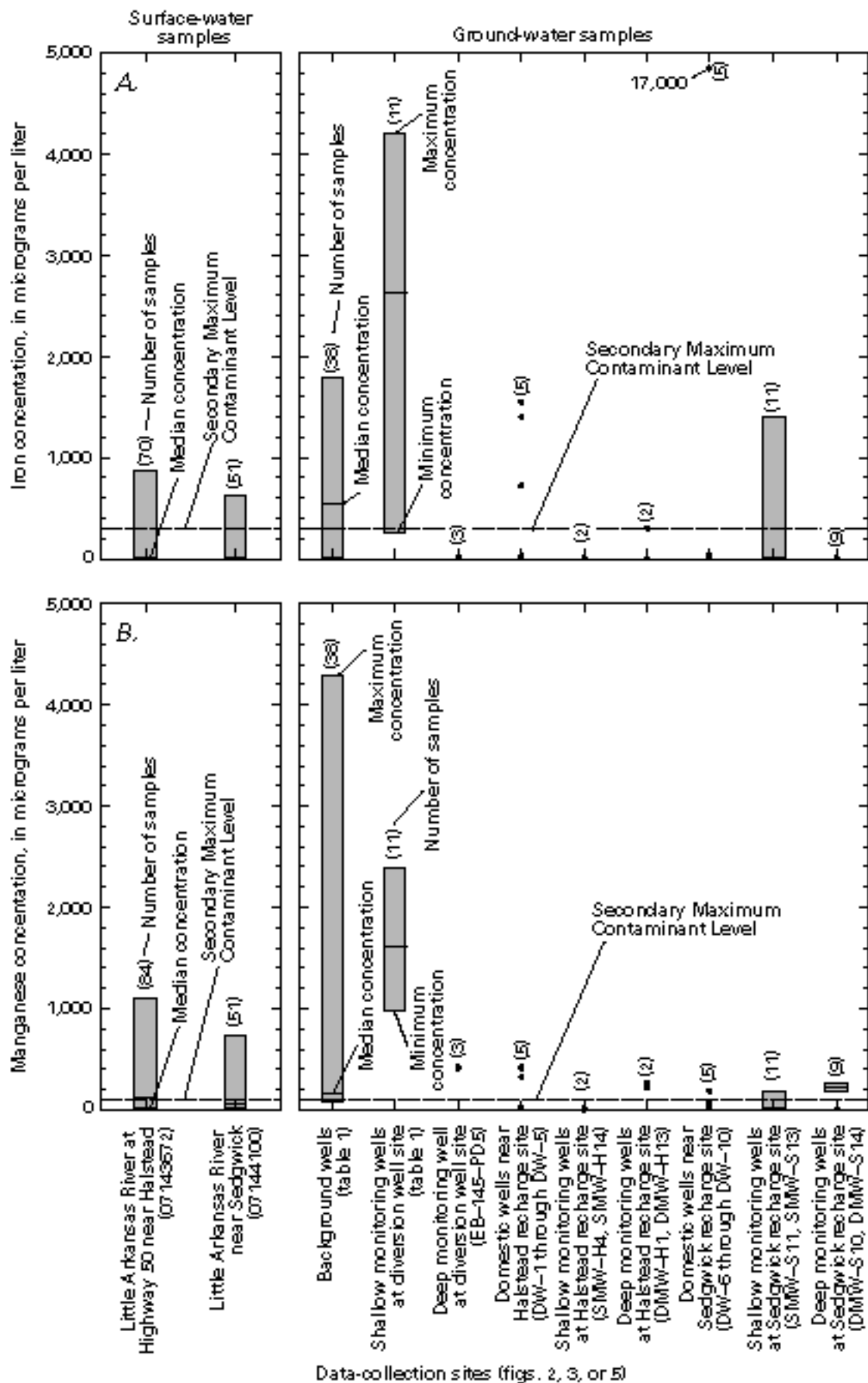
Figure 9. Ranges in (A) iron and (B) manganese concentrations in surface- and ground-water samples during baseline water-quality monitoring. Secondary Maximum Contaminant Levels from U.S. Environmental Protection Agency (1999).
