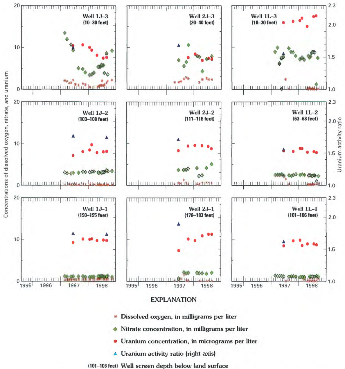
Figure 27. Trends in dissolved oxygen, nitrate, and uranium concentrations, and uranium activity ratios in water from nested wells 1J, 2J, and 1L, Dutch Flats area, 1995 through 1998. Locations of wells are shown in figure 8.
