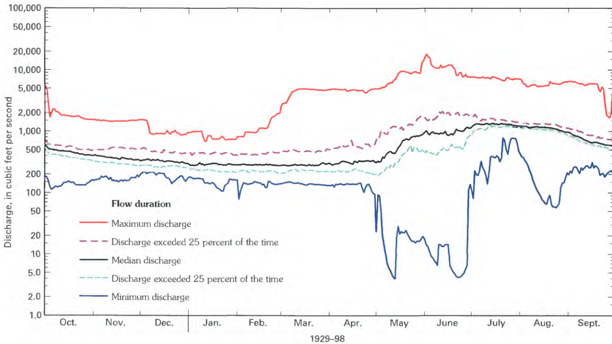
Figure 7. Daily flow duration of North Platte River at Wyoming-Nebraska State line (site SW2, fig. 1), 1929 through 1998.
