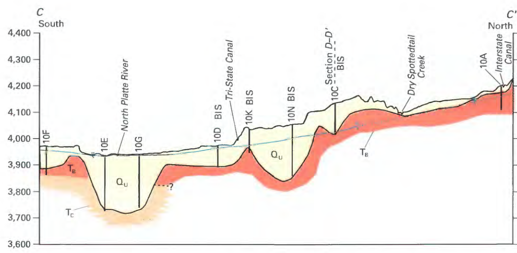
Figure 9. Generalized geologic sections A–A' through D–D' showing principal geologic units transected by ground-water sampling sites and test holes, Dutch Flats area. Traces of sections are shown in figure 8.
