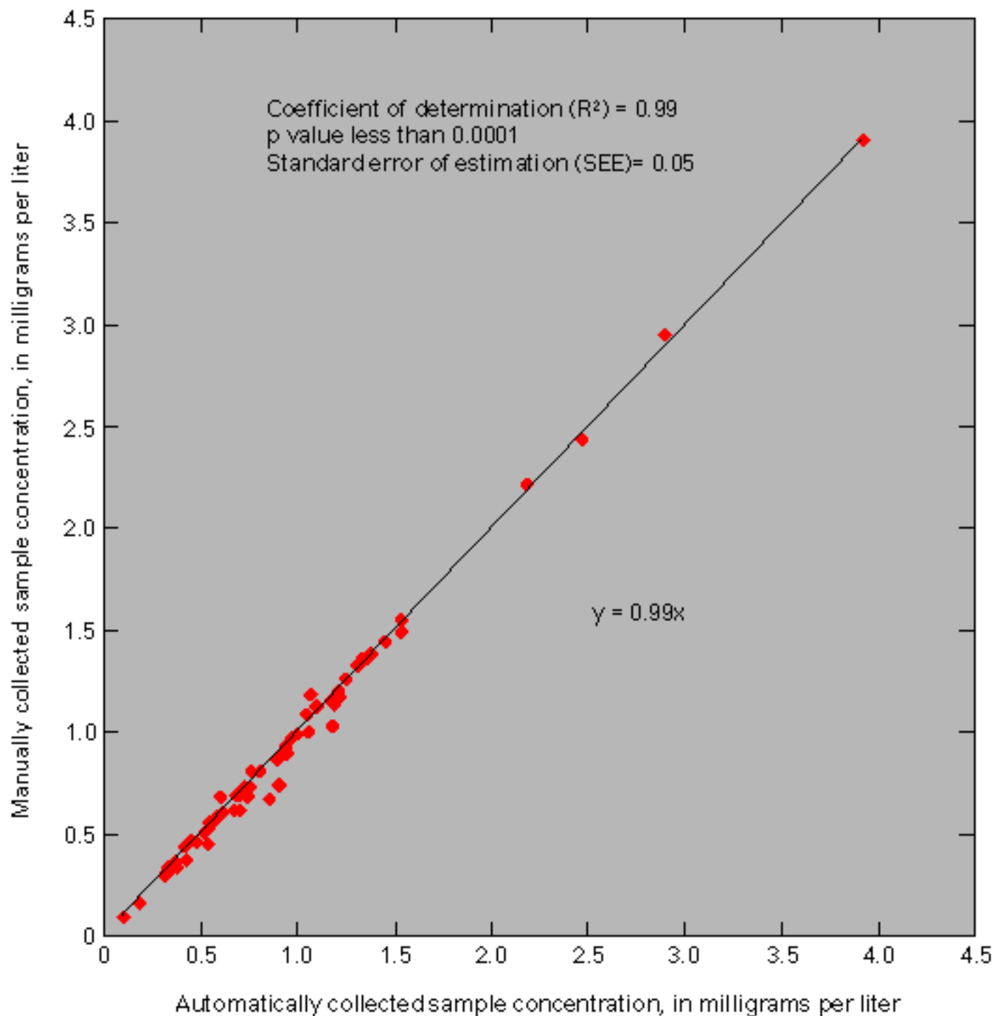
Figure 3. Relation between dissolved nitrate concentrations determined for manually and automatically collected concurrent samples at sampling sites 1-5 in Cheney Reservoir watershed, 1997-2000.
