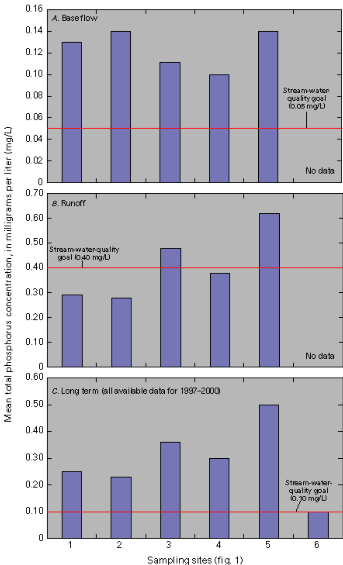
Figure 5. Comparison of mean concentrations of total phosphorus during (A) base-flow, (B) runoff, and (C) long-term streamflow conditions for sampling sites in Cheney Reservoir watershed, 1997-2000. Stream-water-quality goals established by Cheney Reservoir Task Force (written commun., 1996).
