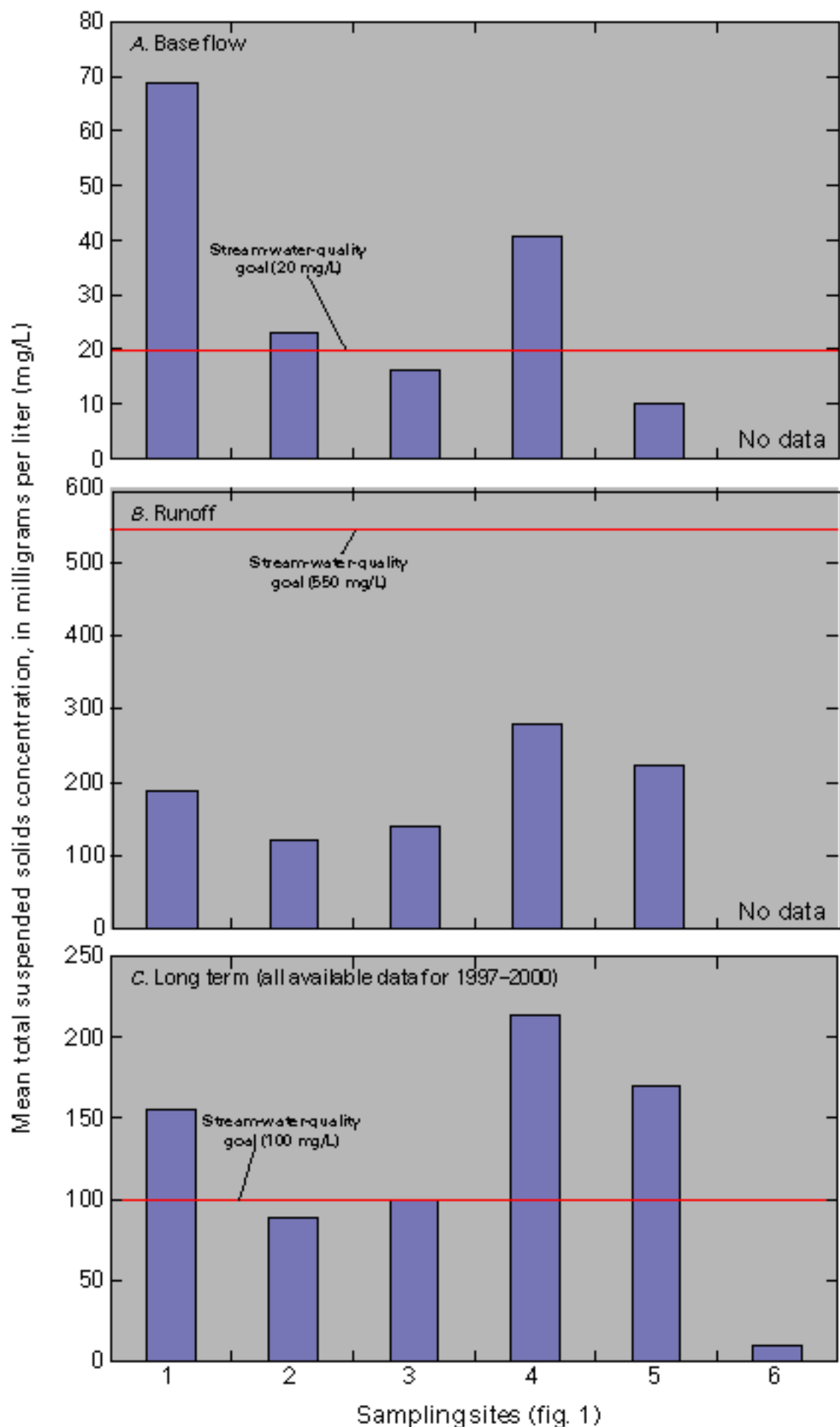
Figure 7. Comparison of mean concentrations of total suspended solids during (A) base-flow, (B) runoff, and (C) long-term streamflow conditions for sampling sites in Cheney Reservoir watershed, 1997-2000. Stream-water-quality goals established by Cheney Reservoir Task Force (written commun., 1996).
