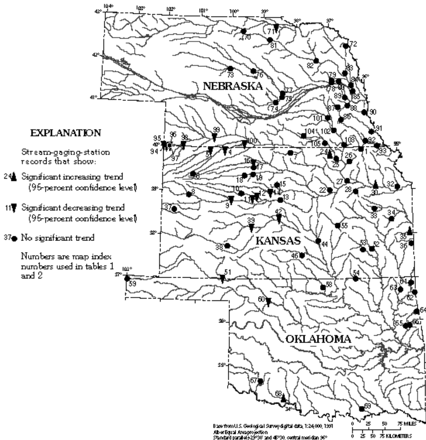
Figure 2. Results of Kendall's tau trend analysis for annual peak flows at selected stream-gaging stations in Kansas, Oklahoma, and Nebraska, 1958-97.
