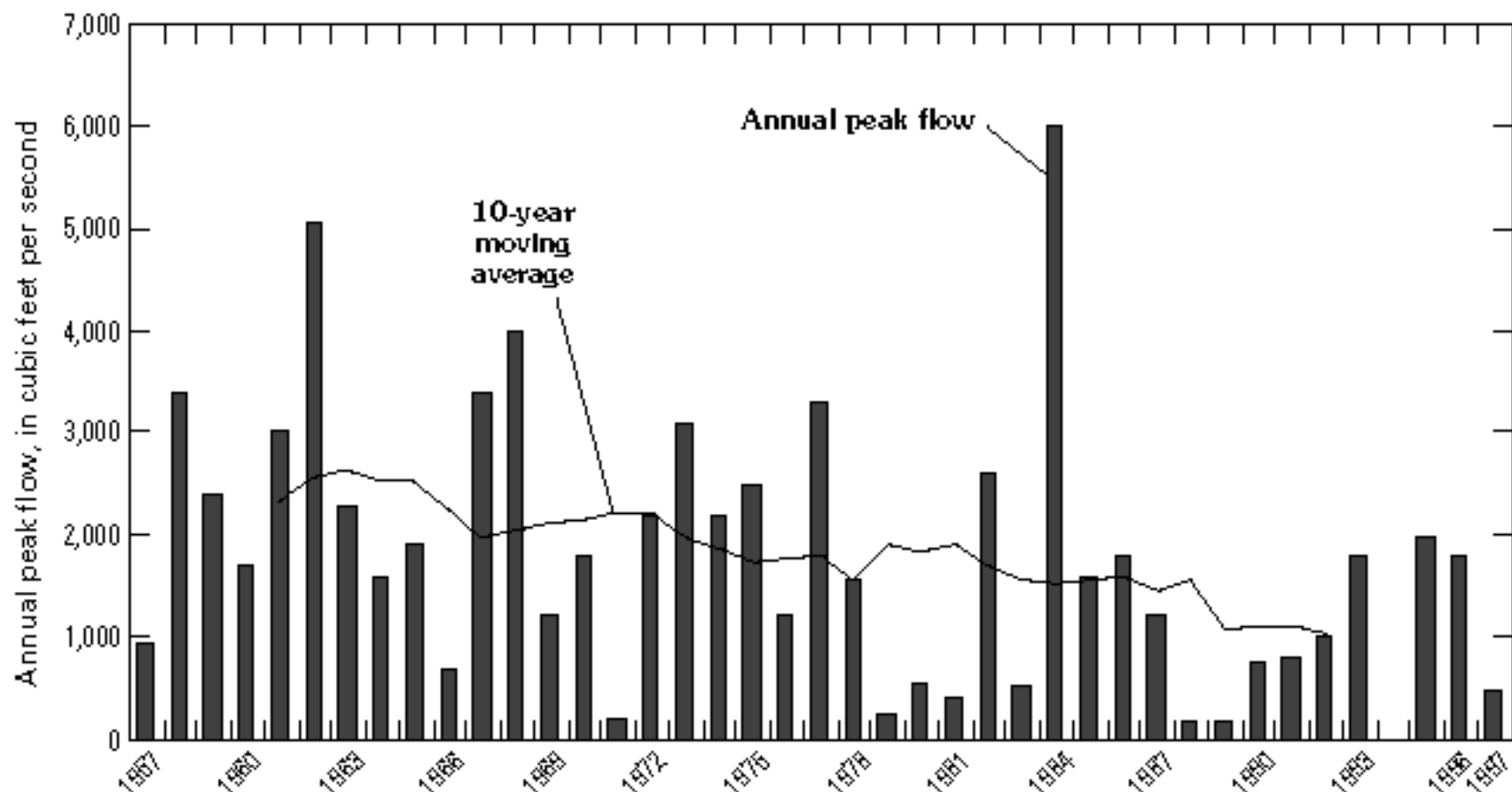
Figure 5B. Annual peak flows and 10-year moving averages using available periods of record—Continued. Location of station shown in figure 3.
