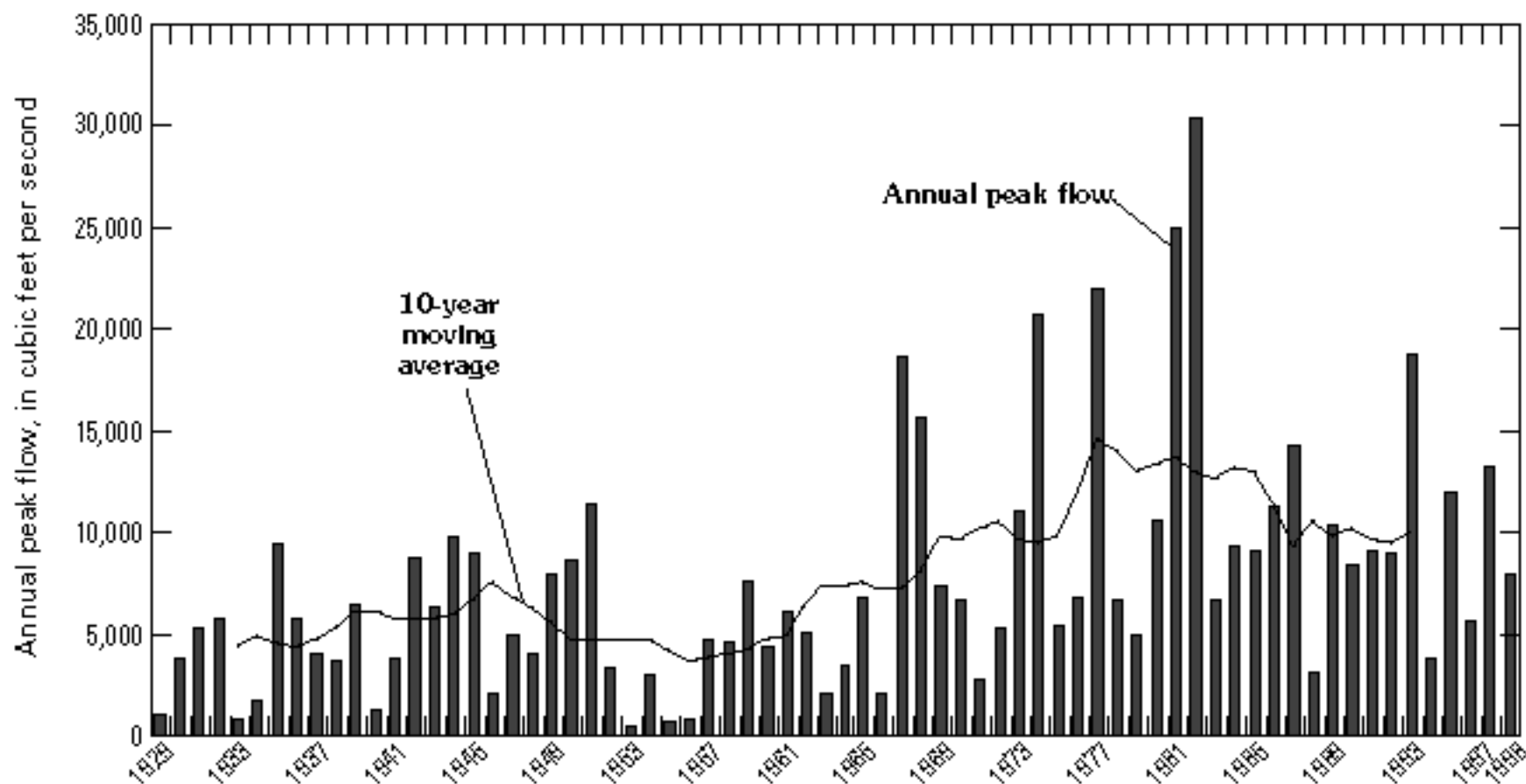
Figure 5CC. Annual peak flows and 10-year moving averages using available periods of record—Continued. Location of station shown in figure 3.
