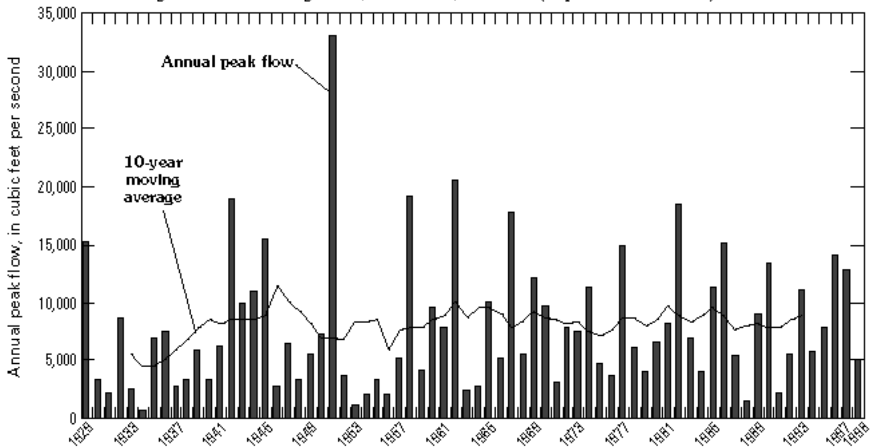
Figure 5DD. Annual peak flows and 10-year moving averages using available periods of record—Continued. Location of station shown in figure 3.
