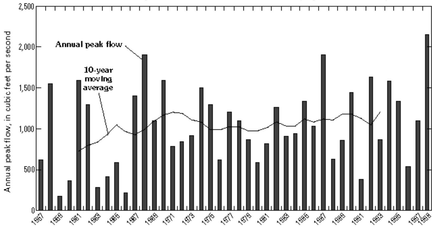
Figure 5HH. Annual peak flows and 10-year moving averages using available periods of record—Continued. Location of station shown in figure 3.
