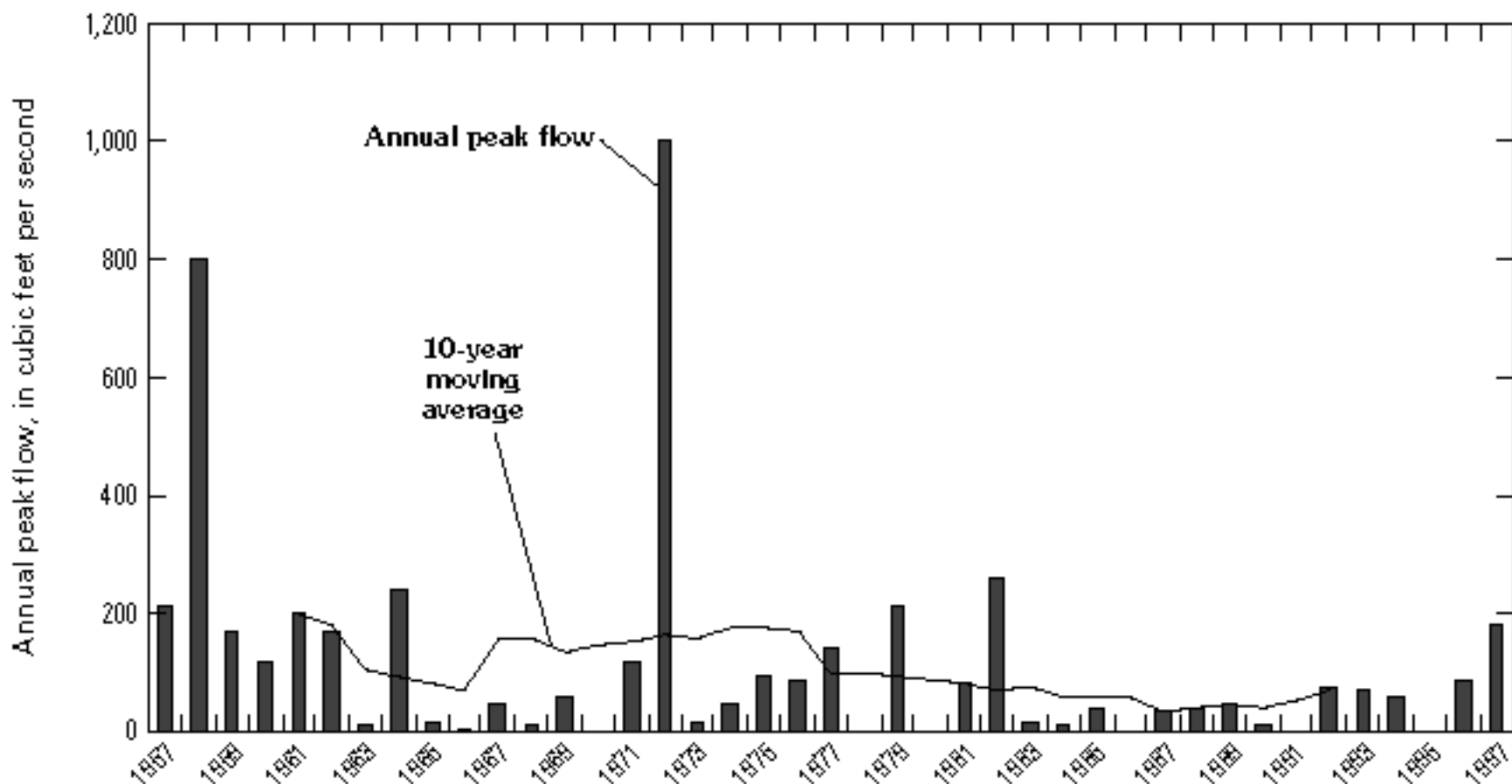
Figure 5// Annual peak flows and 10-year moving averages using available periods of record—Continued. Location of station shown in figure 3.
