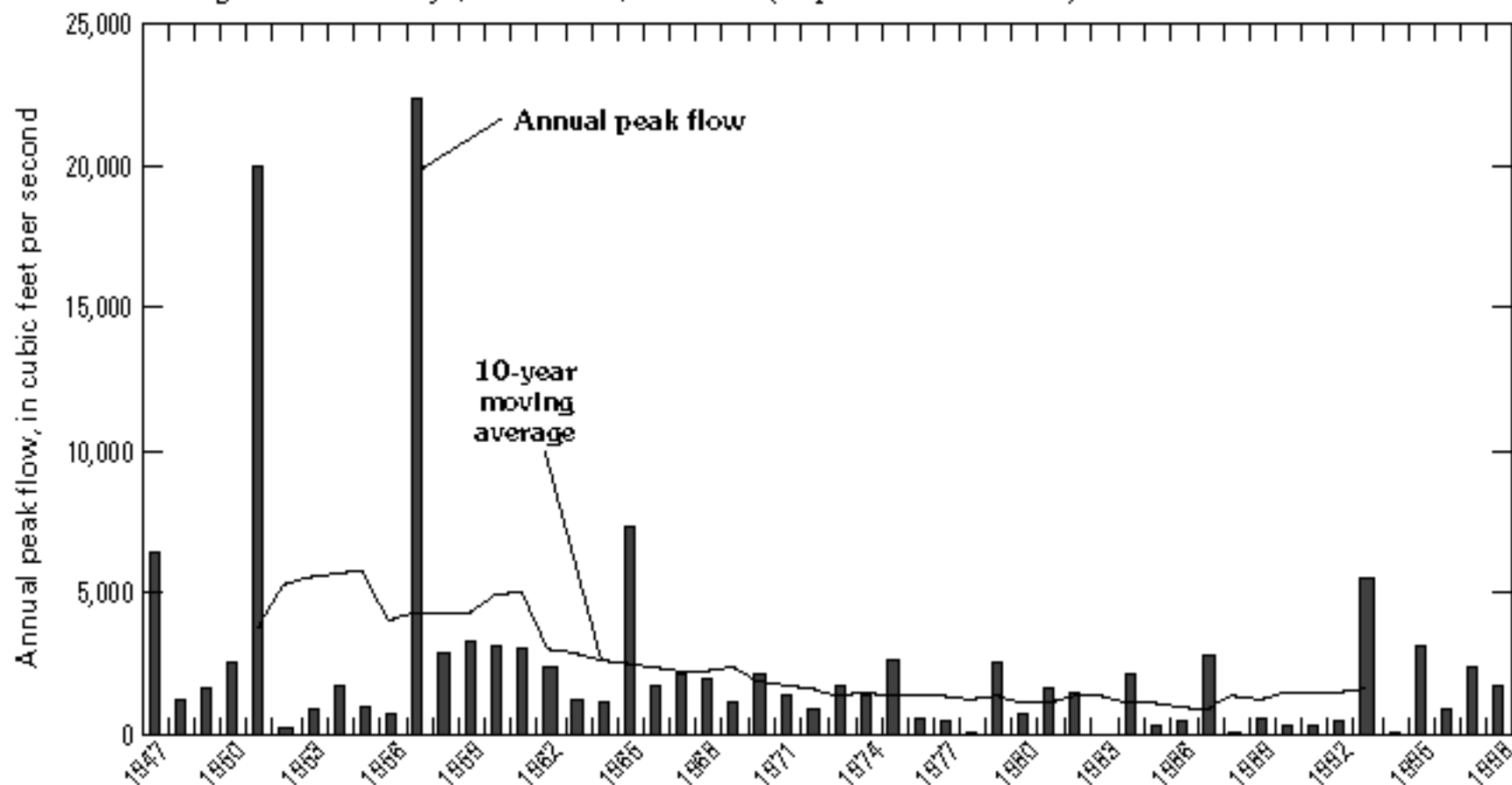
Figure 5K. Annual peak flows and 10-year moving averages using available periods of record—Continued. Location of station shown in figure 3.
