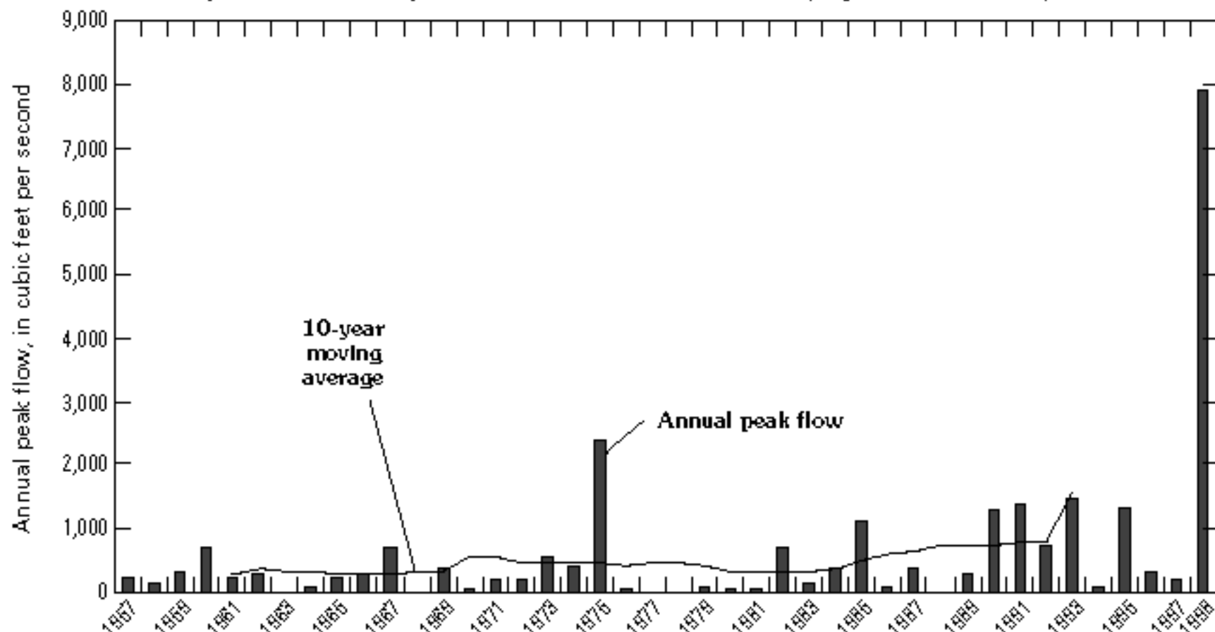
Figure 5M. Annual peak flows and 10-year moving averages using available periods of record—Continued. Location of station shown in figure 3.
