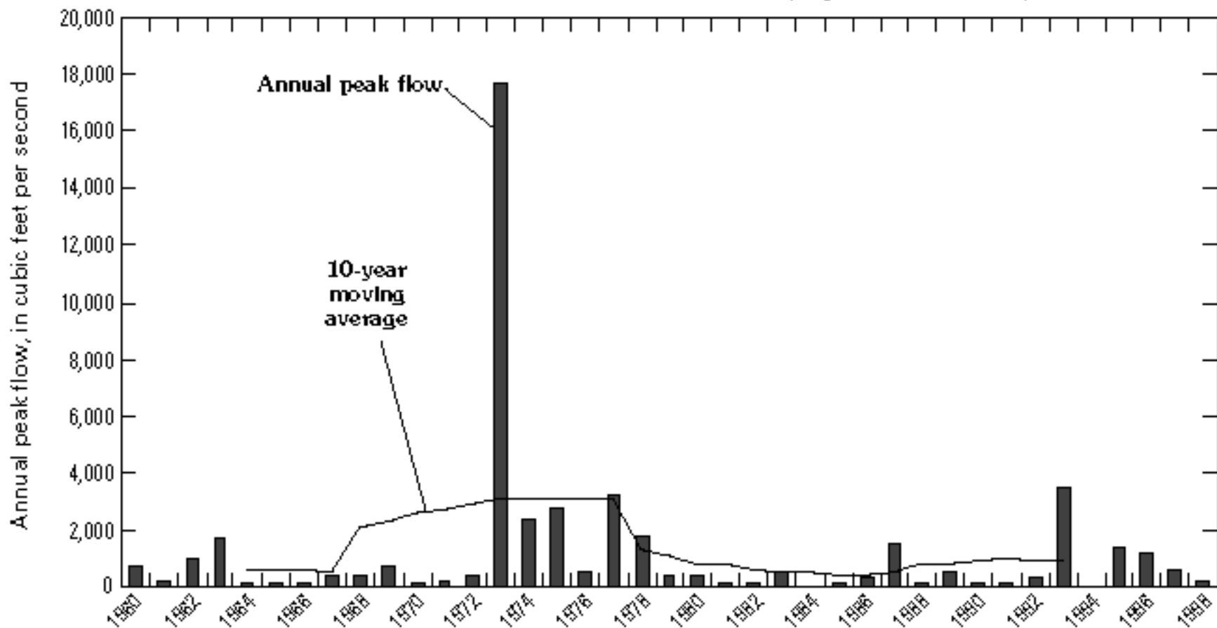
Figure 5MM. Annual peak flows and 10-year moving averages using available periods of record—Continued. Location of station shown in figure 3.
