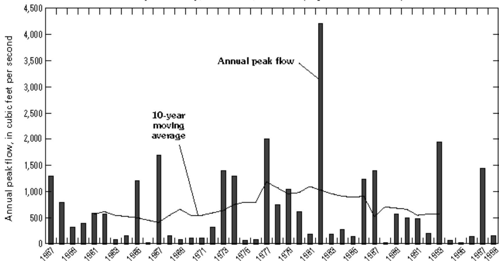
Figure 50. Annual peak flows and 10-year moving averages using available periods of record—Continued. Location of station shown in figure 3.
