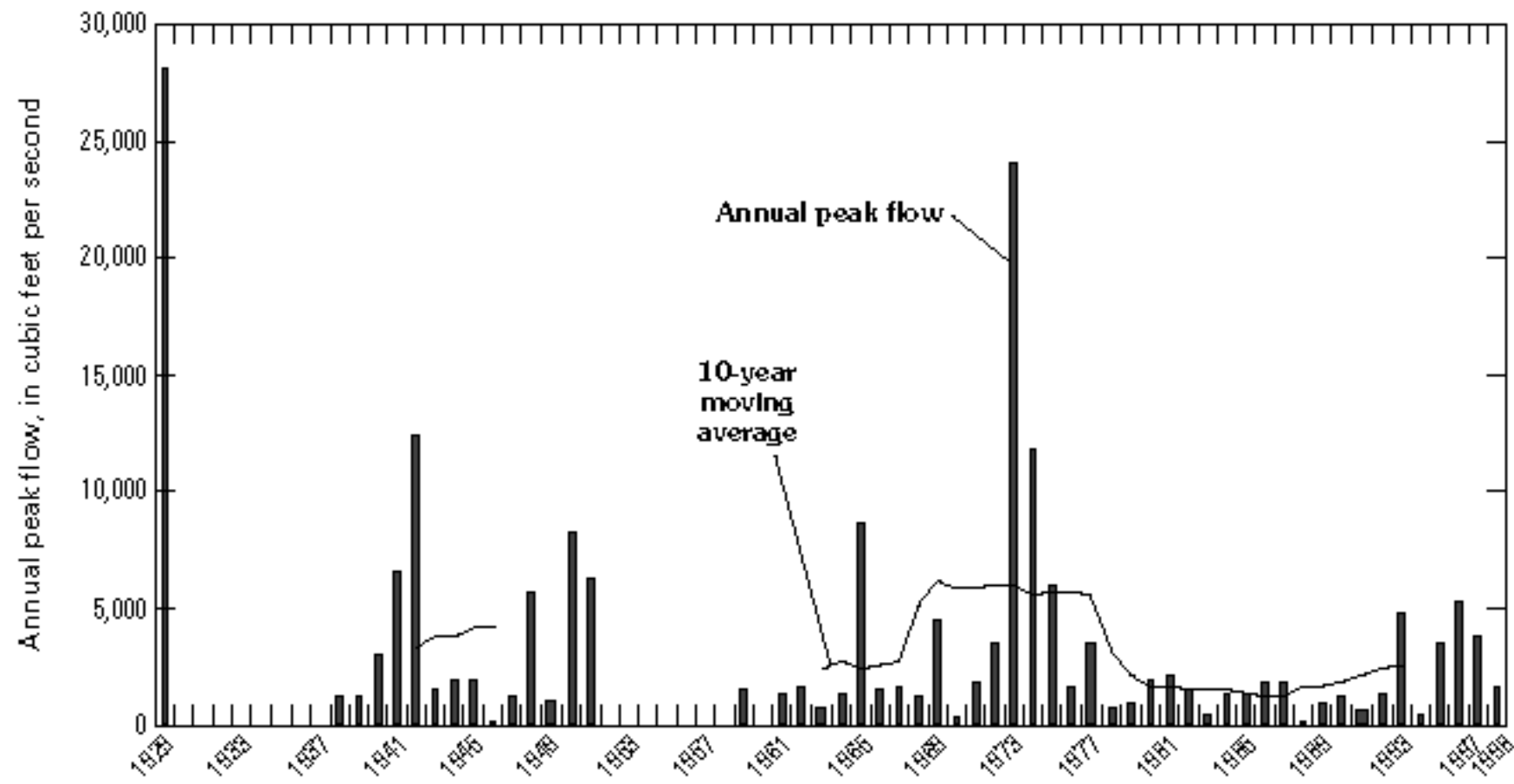
Figure 500. Annual peak flows and 10-year moving averages using available periods of record—Continued. Location of station shown in figure 3.
