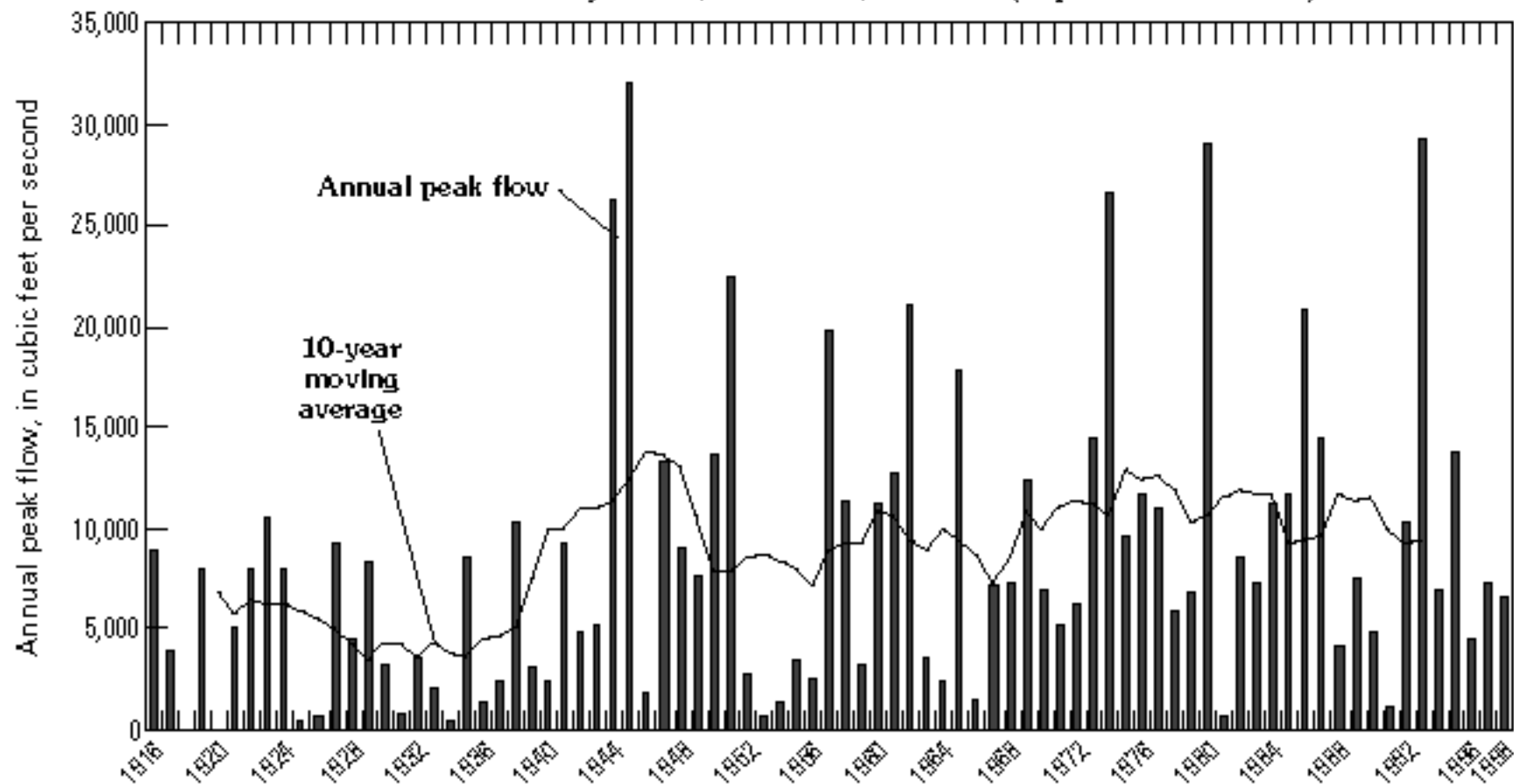
Figure 5PP. Annual peak flows and 10-year moving averages using available periods of record—Continued. Location of station shown in figure 3.
