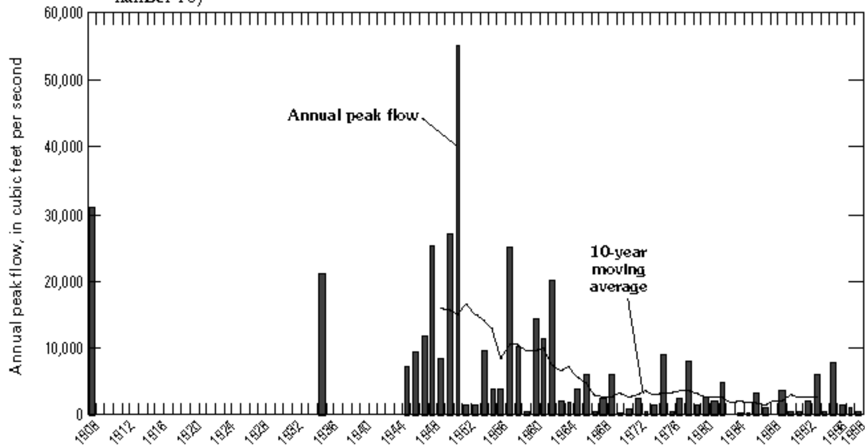
Figure 5R. Annual peak flows and 10-year moving averages using available periods of record—Continued. Location of station shown in figure 3.
