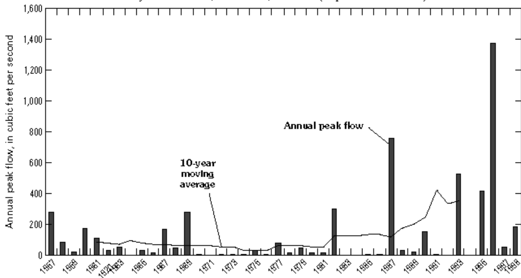
Figure 5S. Annual peak flows and 10-year moving averages using available periods of record—Continued. Location of station shown in figure 3.
