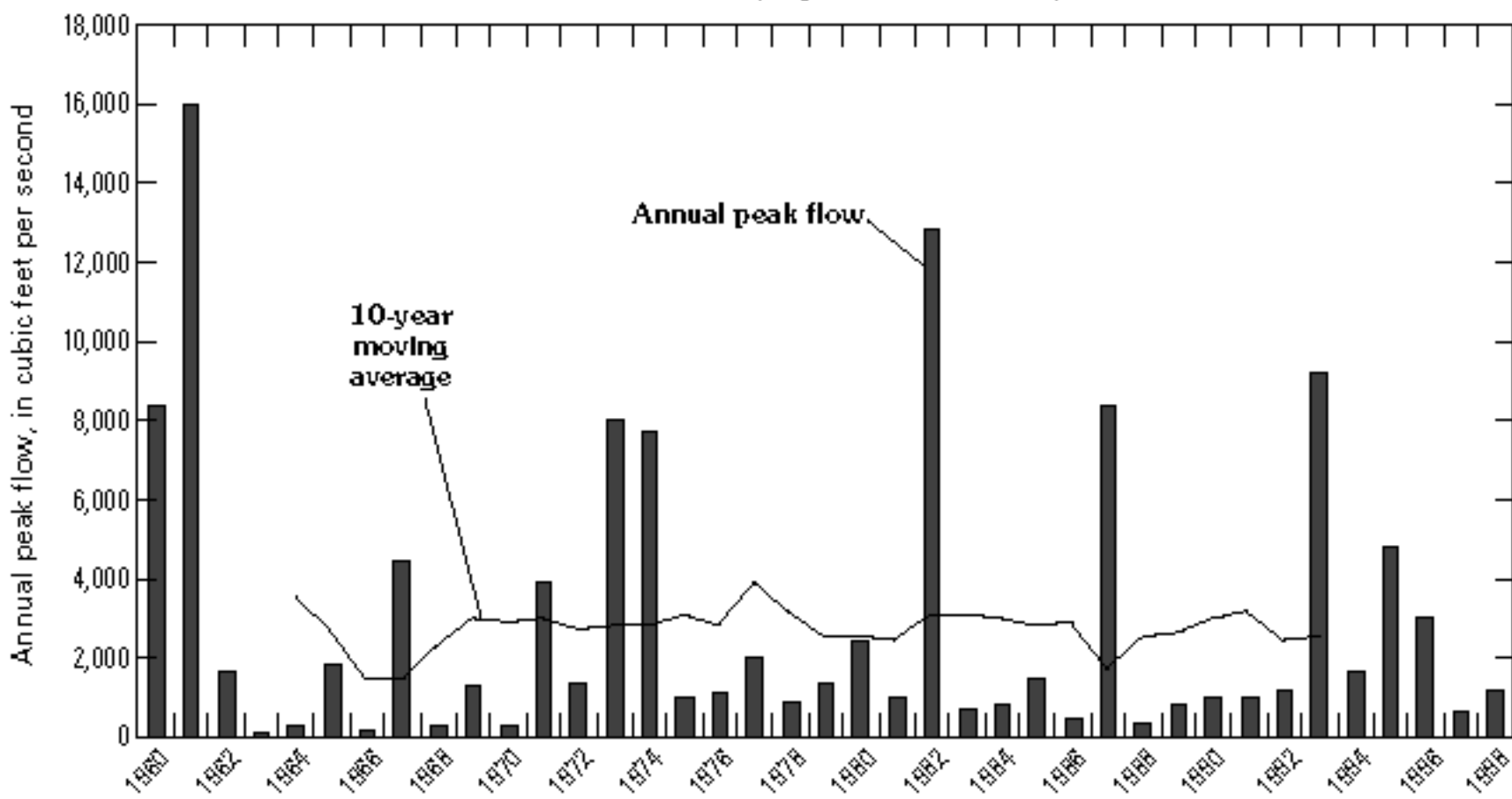
Figure 57. Annual peak flows and 10-year moving averages using available periods of record—Continued. Location of station shown in figure 3.
