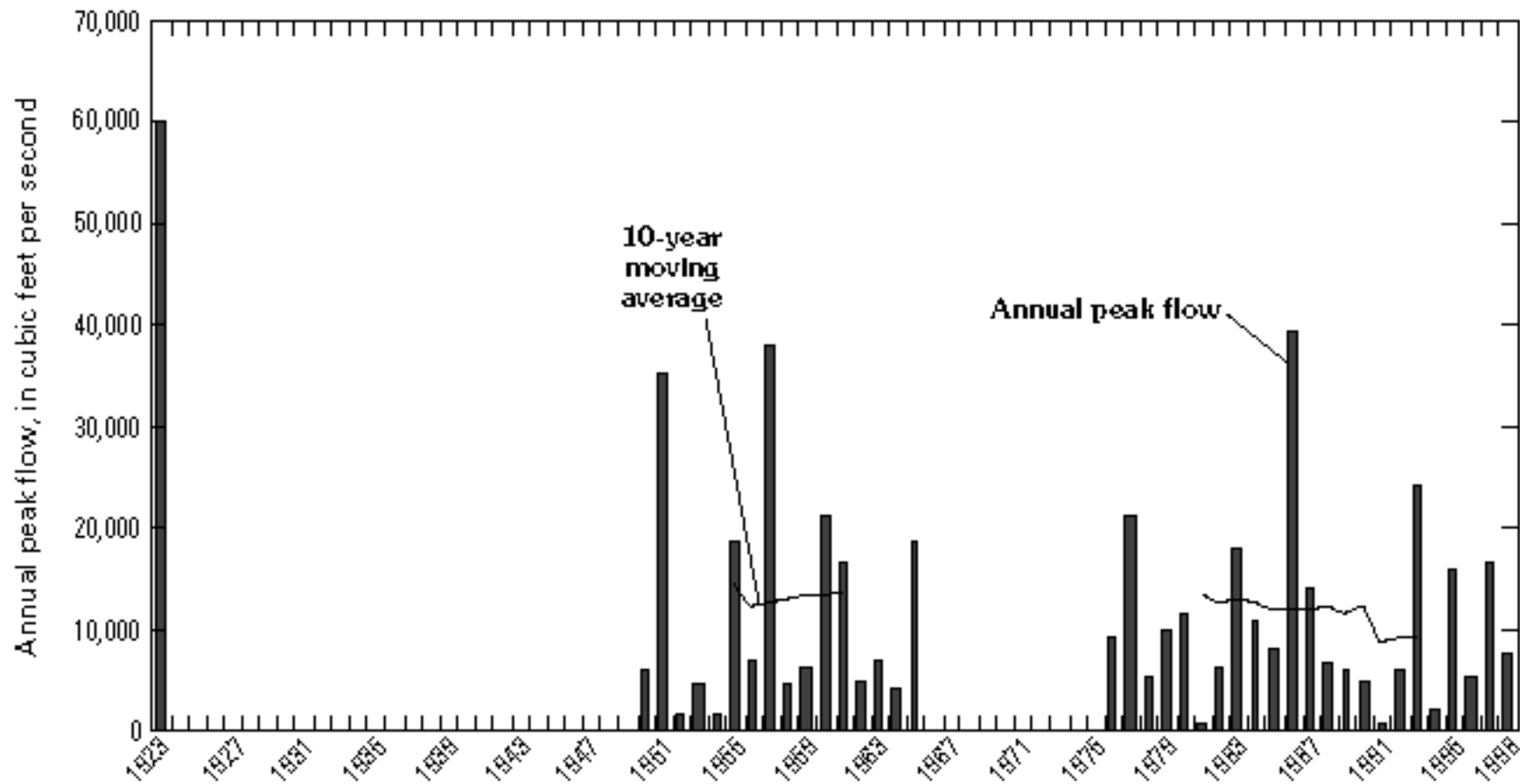
Figure 5UU. Annual peak flows and 10-year moving averages using available periods of record—Continued. Location of station shown in figure 3.
